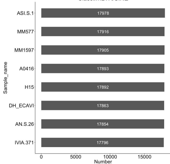
Class//nLTR/SINE
