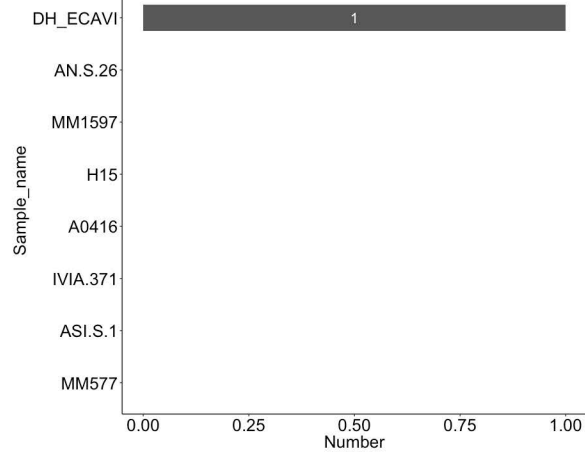
ClassII//DNA_MITE/MuDR
