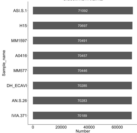
Class//nLTR/LINE
