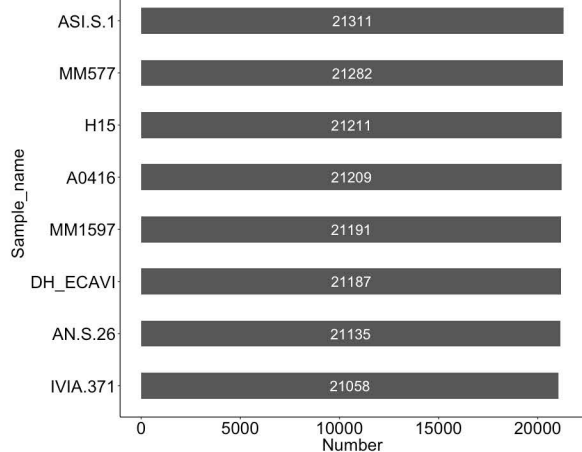
ClassII//DNA_MITE/mites_Others
