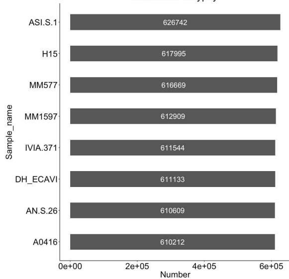
Class//LTR/Gypsy
