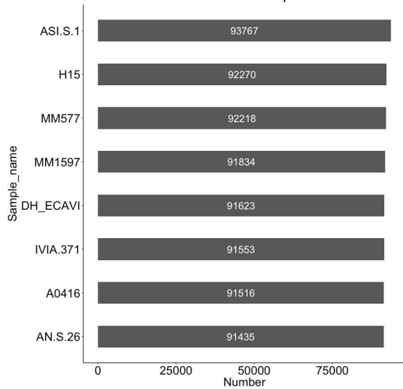
Class//LTR/Copia
