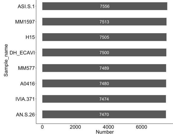
ClassII//DNA_nMITE/EnSpm
