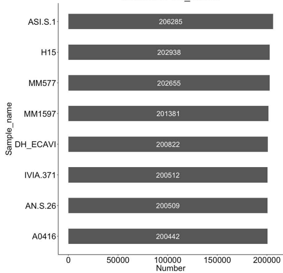
Class//LTR/ltr_Others
