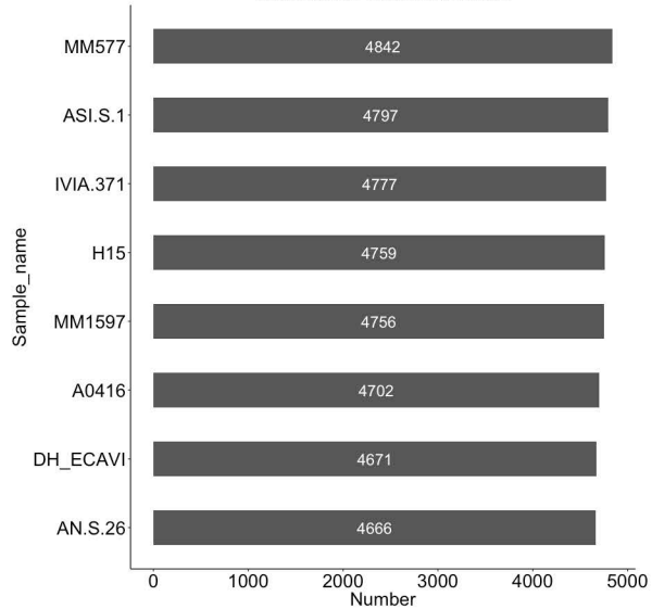
Class//LTR/Caulimovirus
