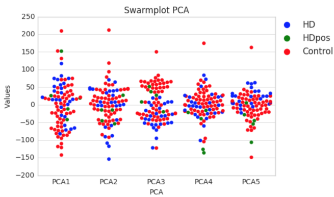
Figure 2. PCA swarm plot of the first five components by % explained variance. No strong outliers were removed based on these projections.
