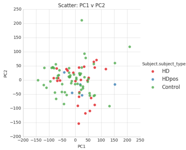
Figure 1. PCA identified no outliers that exerted a strong influence on the results in the first two components.
