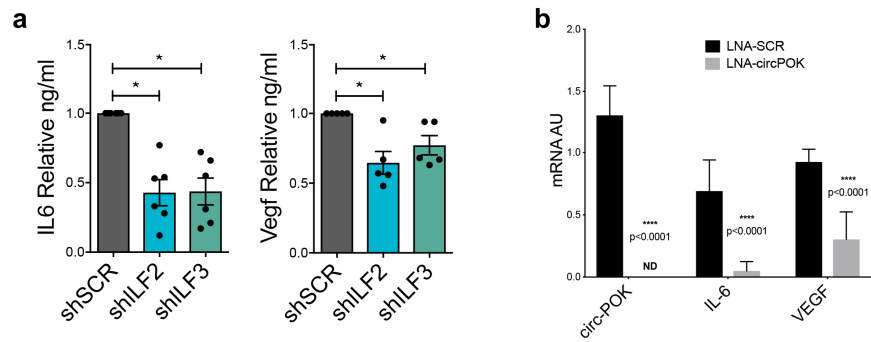
Figure S5. ILF2/3 complex regulate the expression of IL6 and VEGF proteins. a ELISA assays to detect the expression of IL6 (left), and Vegf (right) in the supernatant of p53^{-/-} Zbtb7a\_Ex2^{F/F-CRE} MSCs expressing circPOK-GTG upon knock-down of ILF2 or ILF3. b RT-qPCR to detect the expression levels of circPOK, IL6 and VEGF upon the use of LNA targeting circPOK.
