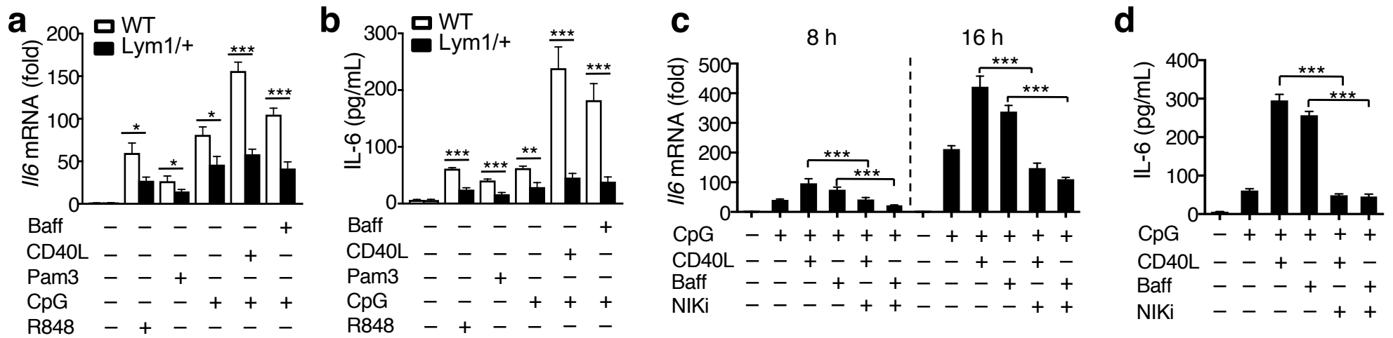
Fig. S7. Induction of IL-6 expression in B cells requires the noncanonical NF- \kappa B pathway. a,b qRT-PCR ( a ) and ELISA ( b ) analyses of IL-6 expression in wildtype (WT) or Nfkb2 lym1/+ splenic B cells that were either not treated (-) or stimulated (+) with the indicated inducers. c,d qRT-PCR ( c ) and ELISA ( d ) analysis of IL-6 expression in wildtype splenic B cells that were stimulated (+) with the indicated inducers either in the absence (-) or presence (+) of small molecule inhibitor of NIK (NIK i , 5 \mu M)
