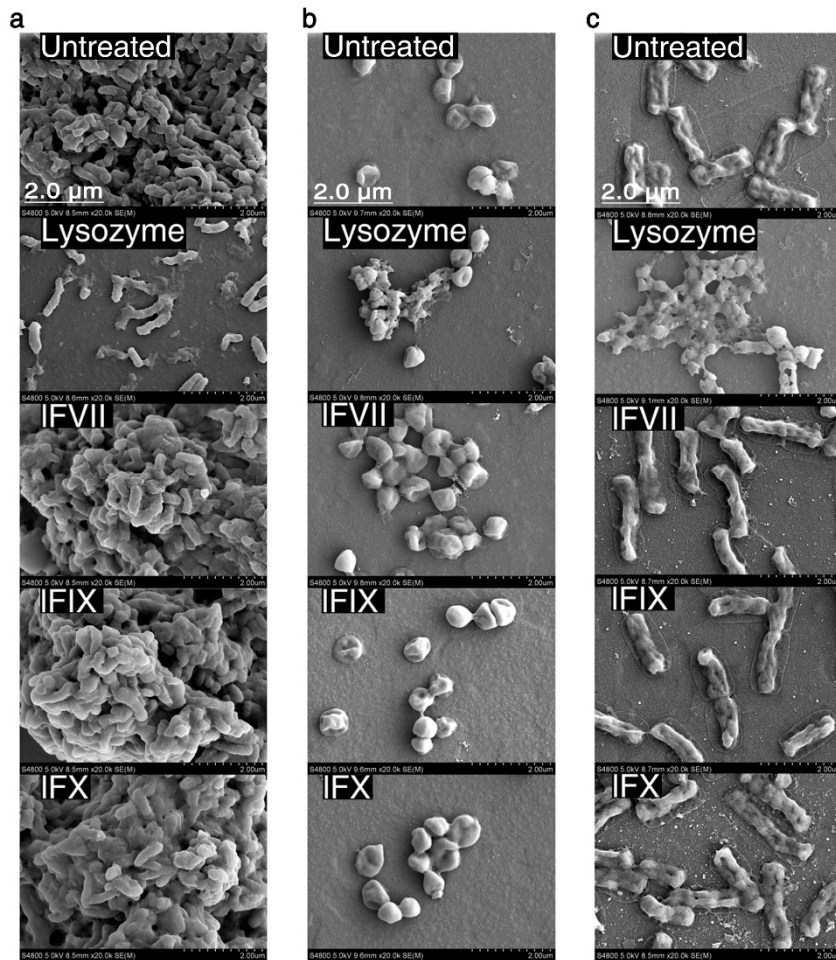
Fig. S3 LCs do not cause the degradation of PGN. PGN of E. coli K12 (a), Staphylococcus aureus (b) and Bacillus subtilis (c) in TBS were incubated for 3 h at 37 °C with the LCs or lysozyme, washed with TBS, and then scanned by SEM. Untreated PGN was included in all experiments. The final concentrations of the LCs and lysozyme are listed as follows: lysozyme, 50 μg/ml; IFVII, 100 μg/ml; IFIX, 100 μg/ml; IFX, 100 μg/ml.
