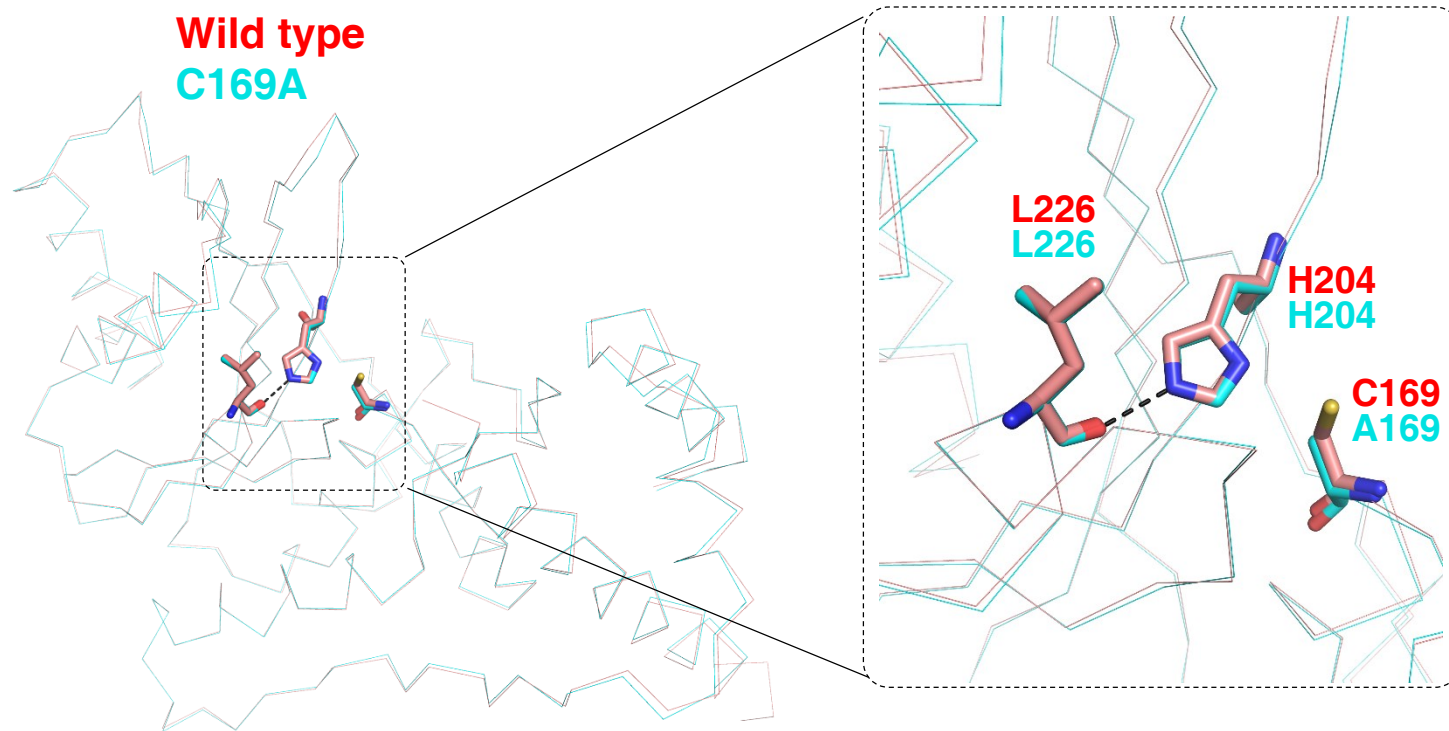
Figure S4. Superposition of structures of wild type VASH1 (red ribbon) and VASH1 C169A (cyan ribbon), with the catalytic-triad residues shown in sticks.
