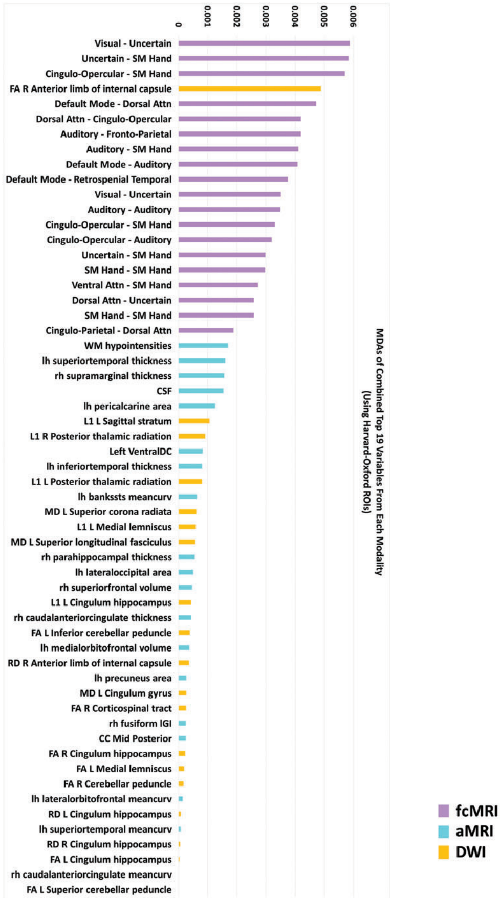
SUPPLEMENTARY FIG. S9. Histogram showing MDAs of the combined top 19 variables from each modality (combined top 57 variables) in analysis 3b (using the fcMRI Harvard-Oxford ROIs).
