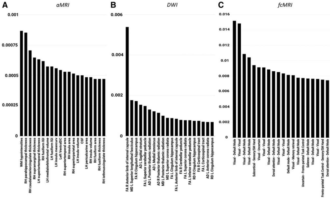
SUPPLEMENTARY FIG. S1. MDAs of the top variables from each modality in analysis 1. For visibility, only the top 20 features from each modality are shown. (A) aMRI; (B) DWI; (C) fcMRI. aMRI, anatomical magnetic resonance imaging; DWI, diffusion weighted imaging; fcMRI, functional connectivity MRI; LH left hemisphere; MDA, mean decrease in accuracy; RH, right hemisphere; WM, white matter.
