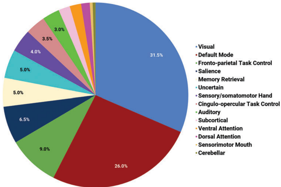
SUPPLEMENTARY FIG. S2. Percentage of participations in the top 100 fcMRI variables by functional network (using network assignments from the study by Power et al., 2011).
