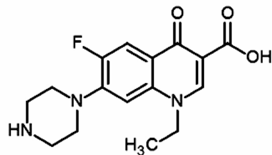
Norfloxacin
