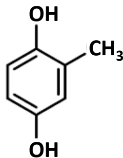
2-Methylhydroquinone
