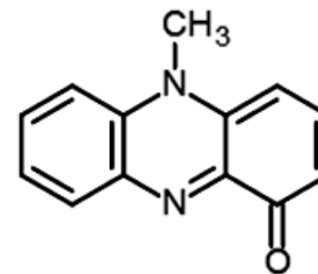
Pyocyanin
