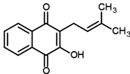
Lapachol
