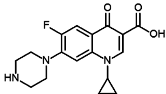
Ciprofloxacin
