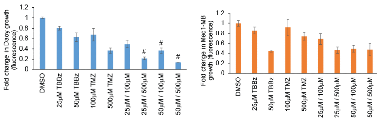
Supplementary Figure S6. Combinatorial treatment of Daoy and Med1-MB cells with CK2 inhibitors and TMZ.
