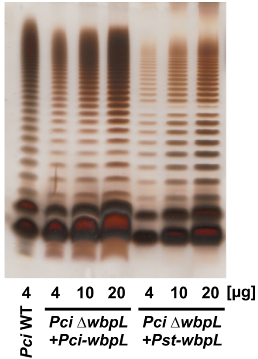
Figure S1: 12% Bis-Tris NuPAGE gel and silver staining of lipopolysaccharide (LPS) preparations from Pseudomonas cichorii ATCC10857/DSM50259 ( Pci ) wild-type (WT), \Delta wbpL :: Gm R ( \Delta wbpL ) deletion mutant strains complemented with plasmid-expressed wbpL ortholog from either Pci (+ Pci-wbpL ) or Pst ( Pst-wbpL ). LPS was isolated by hot phenol-water extraction followed by a phenol-chloroform-petroleum ether extraction. The amount of applied LPS is indicated below the respective lane.
