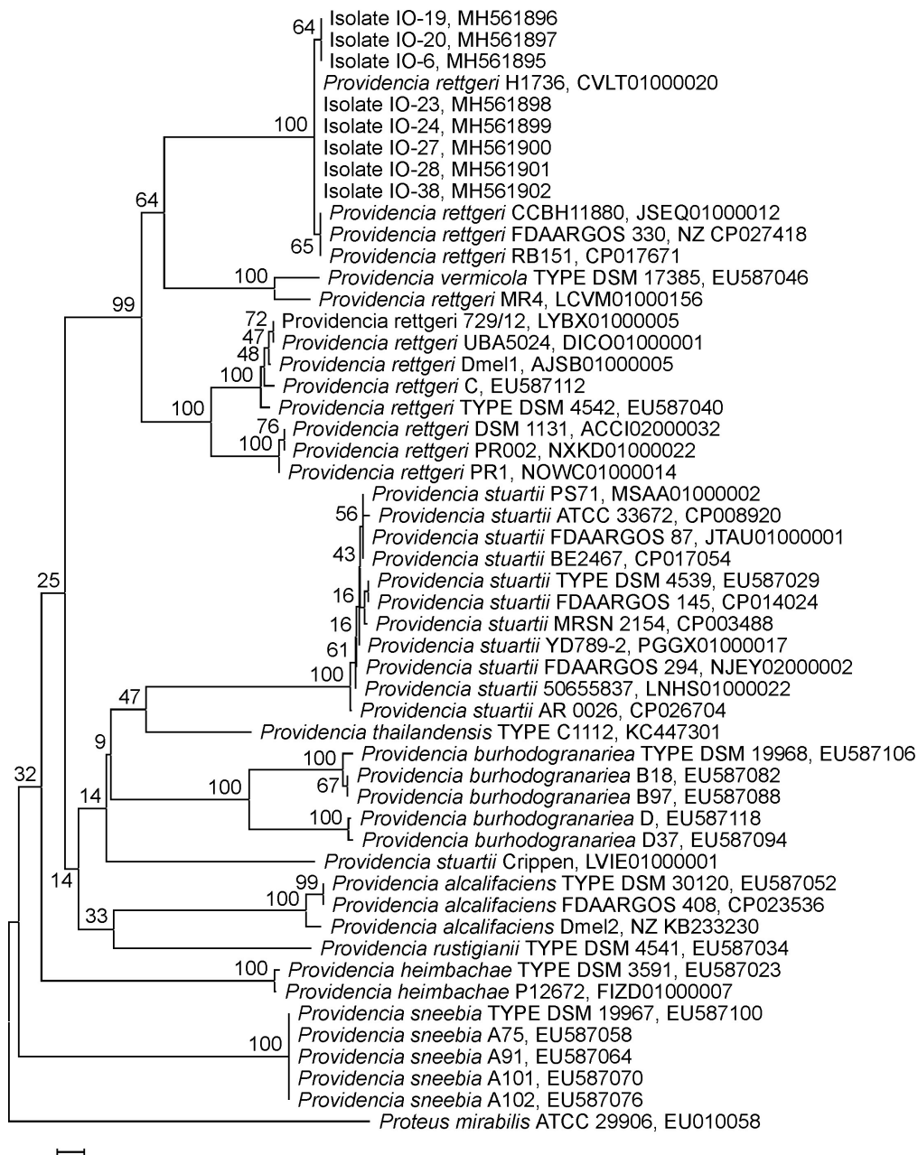
S7 Fig. leuS gene NJ tree. Neighbor Joining (NJ) phylogeny of Providencia bacteria as reconstructed from leuS gene sequences. Terminal branches are labelled by genus, species and strain designations as well as GenBank accession numbers. Numbers on branches indicate bootstrap support values. The size bar corresponds to 1 % sequence divergence. An orthologous sequence from the closely related bacterium Proteus mirabilis has been used as outgroup.
