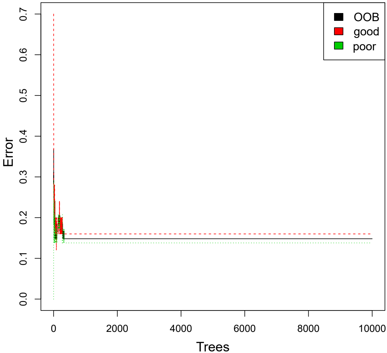
Figure S2: Performance of the random forest model. The plot shows the performance of the random forest model as a function of the trees built in the model, using the generalized OOB (black) and classification error for the good (red) and poor (green) prognosis groups.
