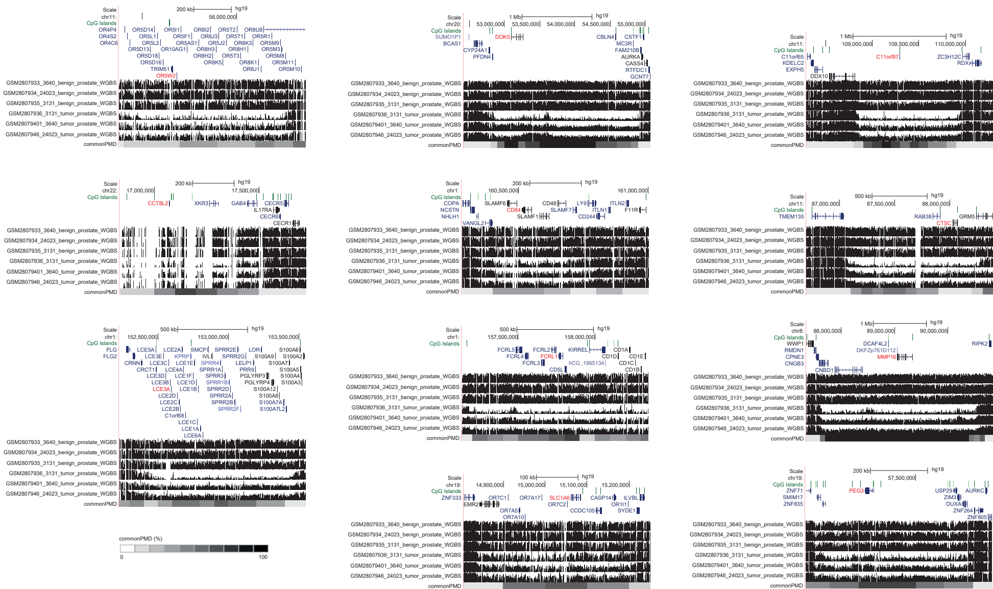
Figure S4: Localization of DMS in PMDs identified in prostate cancer by WGBS. WGBS data for three prostate cancer cases with matching benign tissue was derived from GSE104789 and uploaded to the UCSC genome browser. For comparison, common PMDs identified in eight common cancer types excluding prostate cancer [22] were displays in a color gradient from light grey to black.
