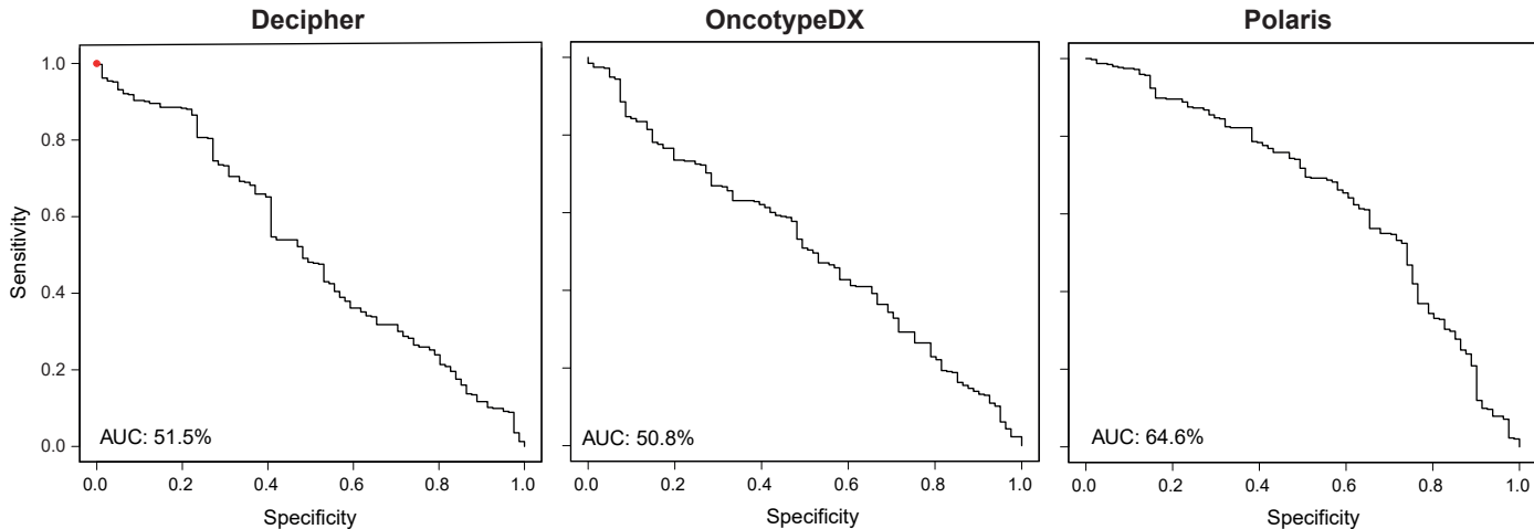
Figure S5: Specificity and sensitivity of gene expression-based prognostic tests to prognosticate PSA-based BCR for the TCGA PRAD cohort. Sums of Z-scores of RNA-seq-derived gene expression per patient was used for calculations of risk scores, as described in Ref. [42].
