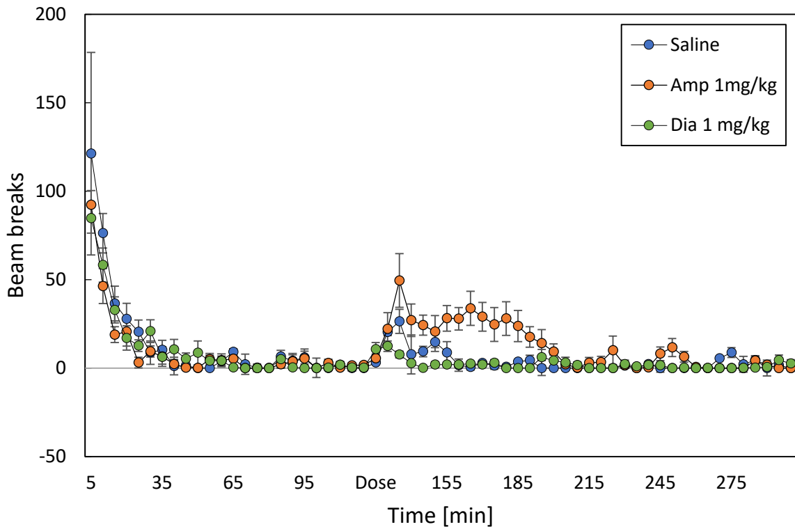
Supporting Figure 2: Changes in activity level induced d-amphetamine (Amp), diazepam (Dia), and saline as assessed by infrared beam breaks in male Wistar rats (n = 8 in each drug-group). Beam breaks were counted within time-intervals of 5 minutes during 5 hours. Drugs were administered after 2 hours of habituation ('Dose' indicates time of dosing).
