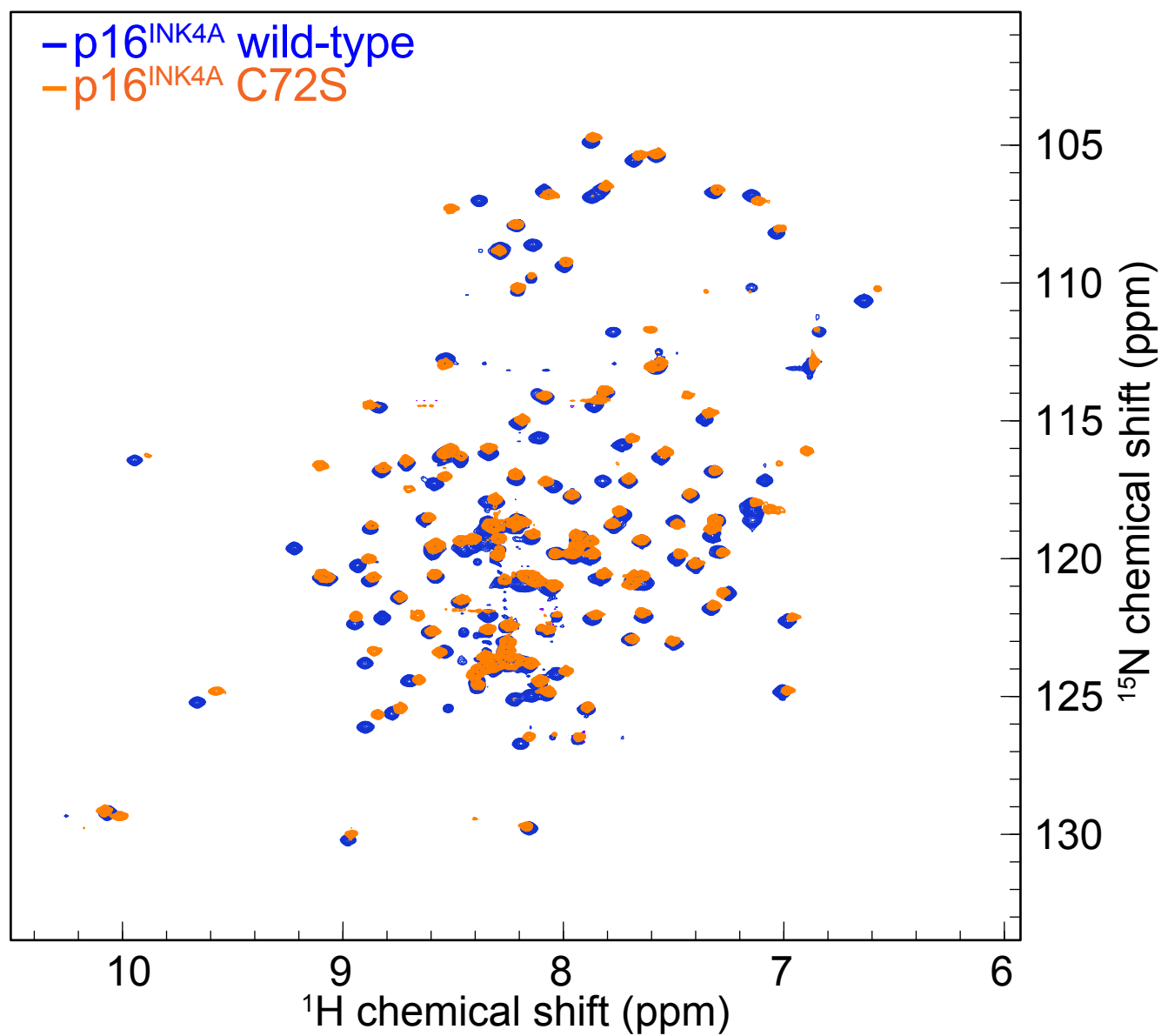
Figure S5. ^1\text{H}^{15}\text{N} HSQC solution NMR spectra of WT p16 INK4A (blue) and p16 INK4A C72S (orange).
