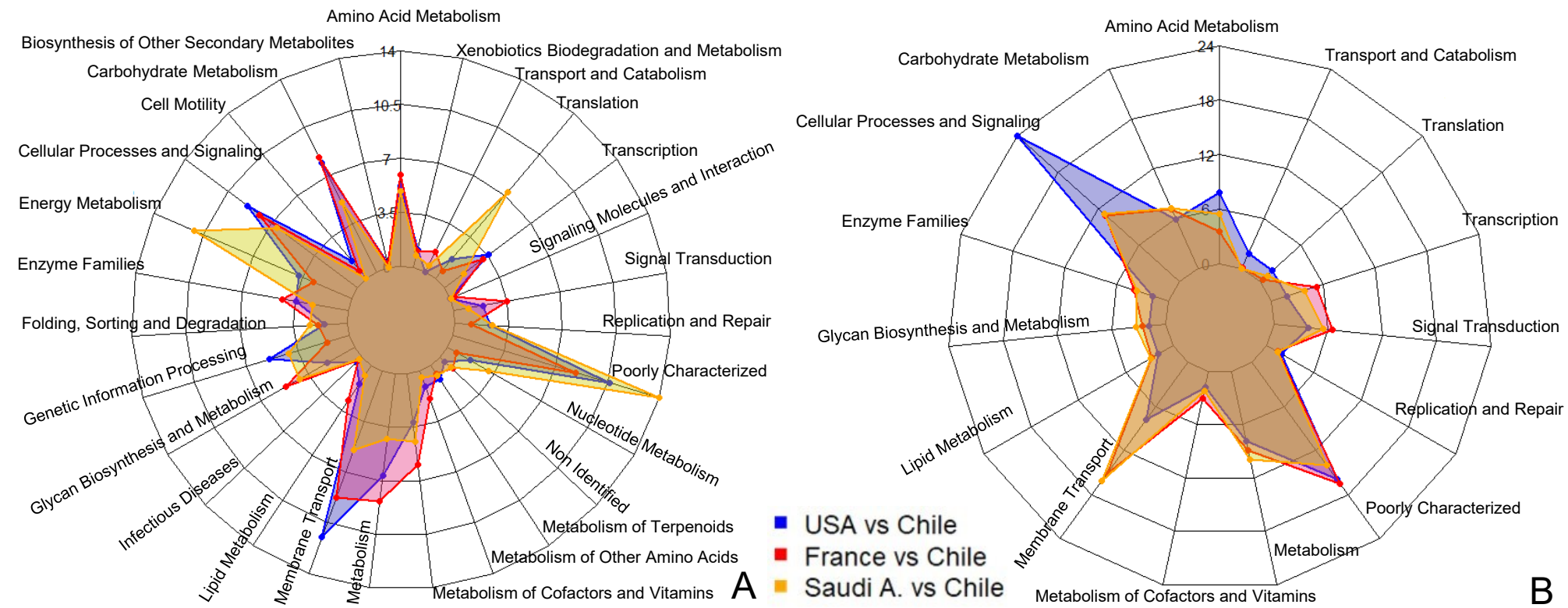
Supplementary Figure 3. Metagenomic assembled pathways from Kegg Orthology simulated data. Spider plot showing relative abundance of significantly downregulated (A) and upregulated (B) metabolic pathways shared between USA (blue), France (red) and Saudi Arabia (yellow) contrasted with Chile. Statistical differences were considered as FDR-adjusted p-value below of 0.05.
