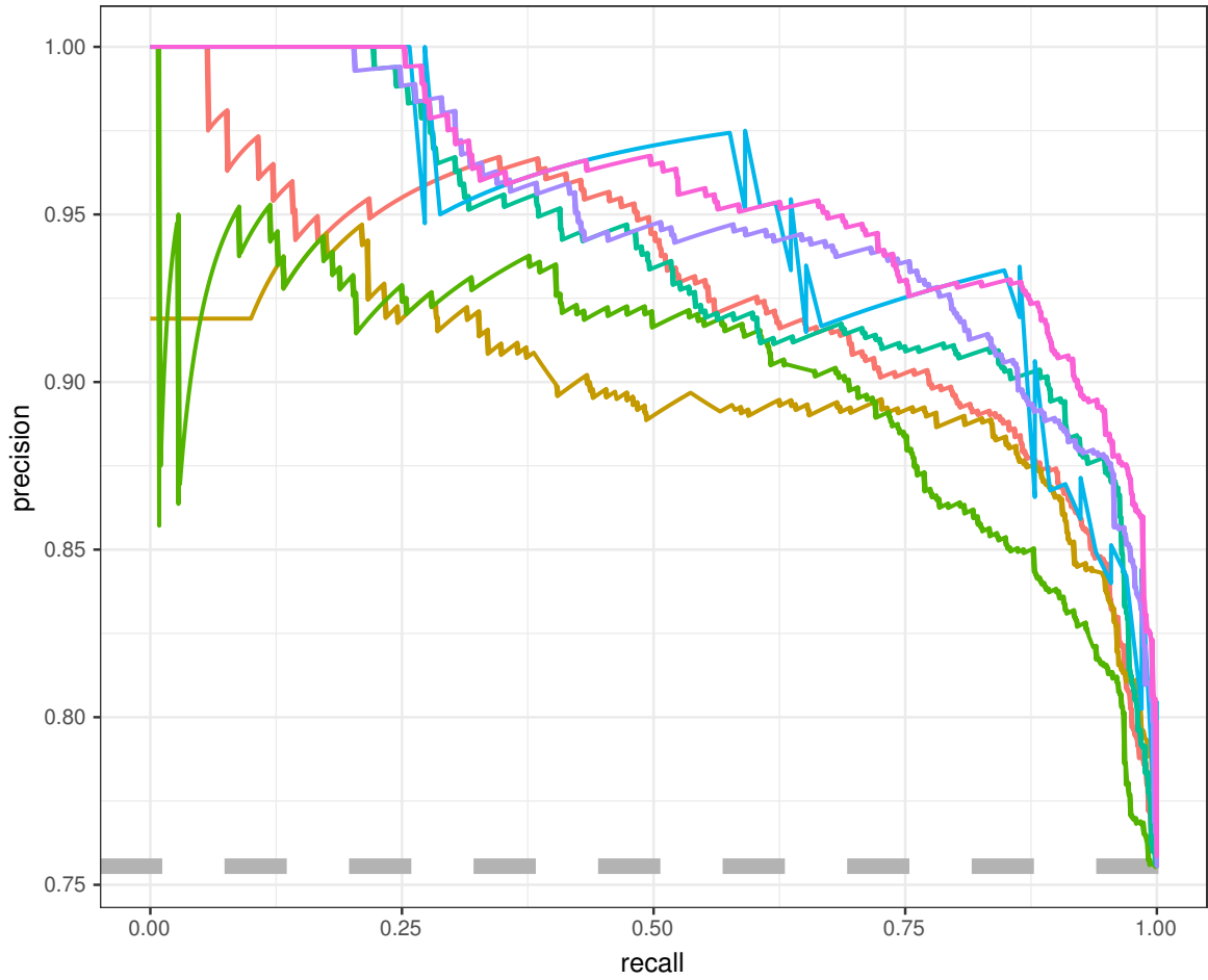
PR Curves
