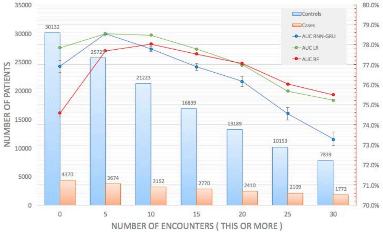
Figure A1: Prediction performance as a function of data density. All features are used in all models. Experiments are limited to a 2 year observation window and 1 year prediction window. All data domains were used. Values are recorded as AUC of prediction.
