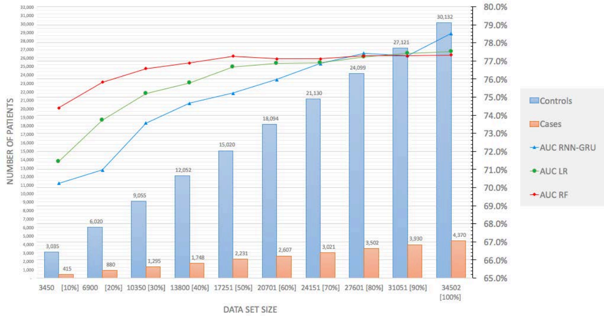
Figure A2: Prediction performance as a function of training set size. All features are used in all models. Values are recorded as AUC of prediction.
