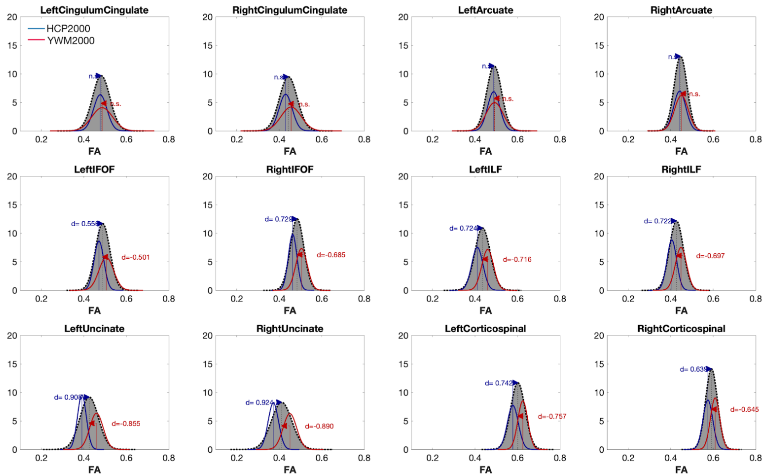
Figure S3b. Normalized probability distributions for the mean FA values, for all tracts and b=2000 experiments.
