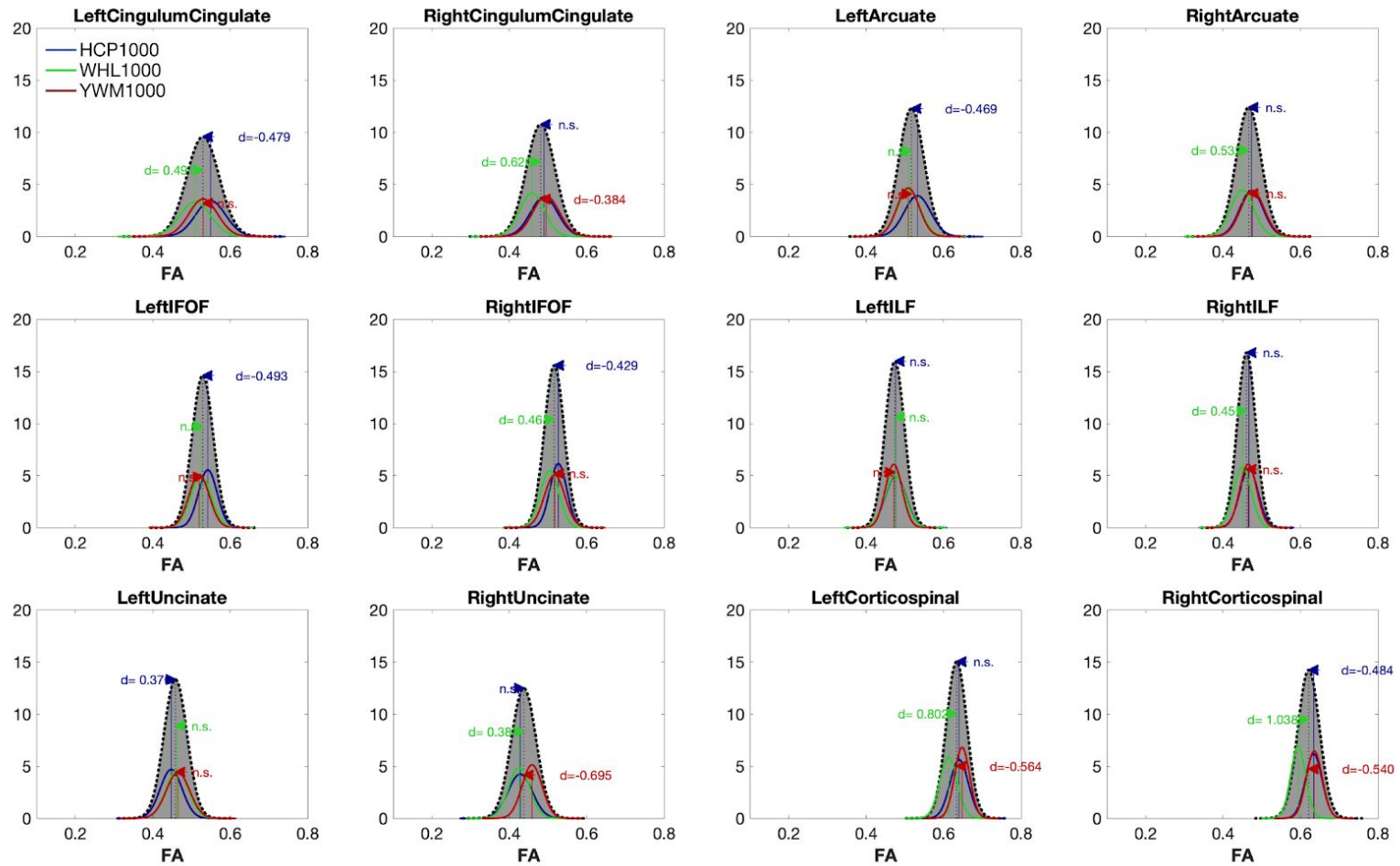
Figure S3a. Normalized probability distributions for the mean FA values, for all tracts and b=1000 experiments.
