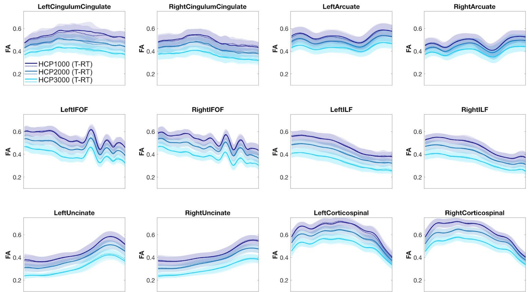
Figure S1a. Average FA profiles, HCP TEST-RETEST experiments, for six homologous white matter tracts.
