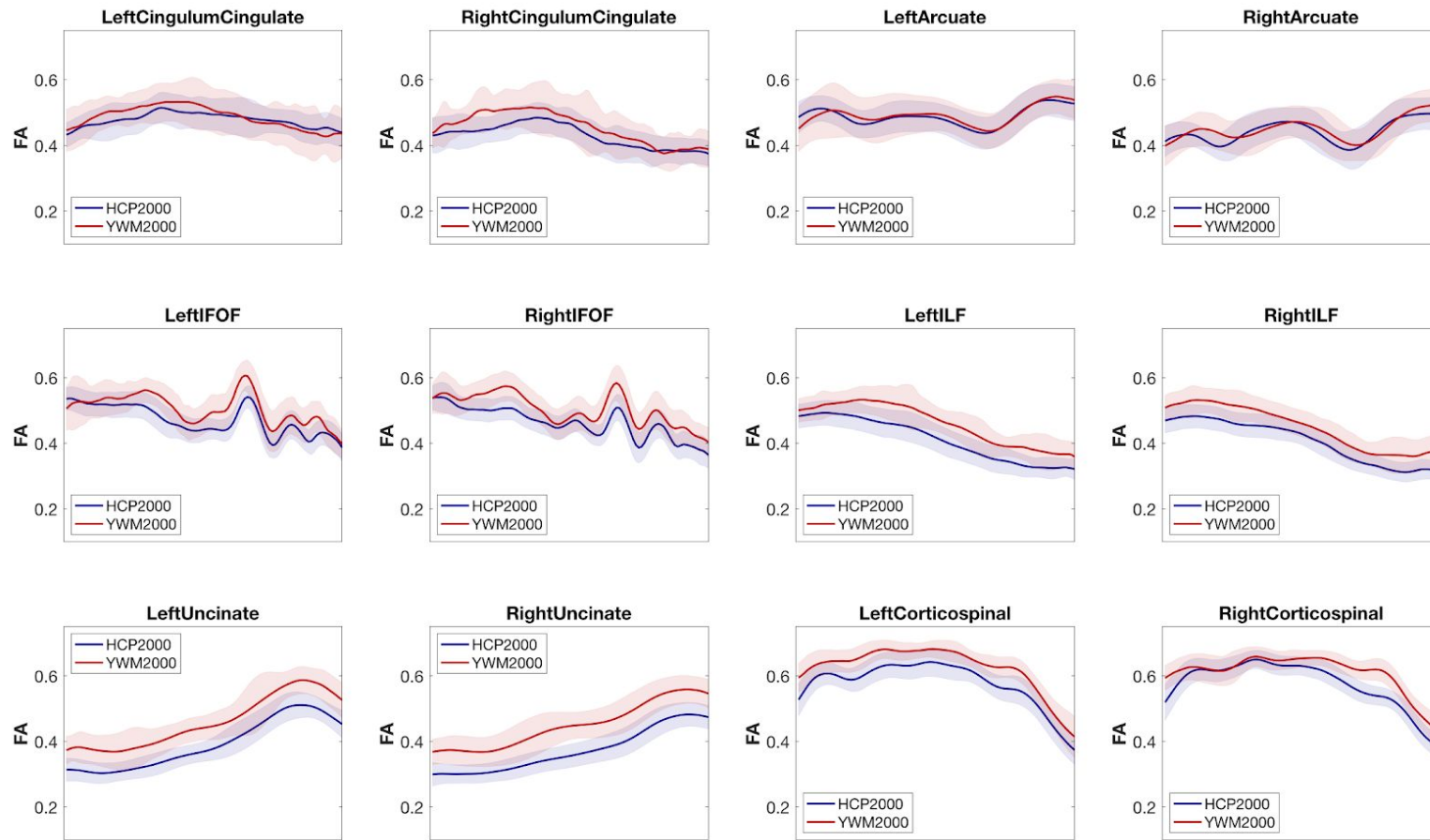
Figure S1c. Average FA profiles, b=2000 experiments, for six homologous white matter tracts.
