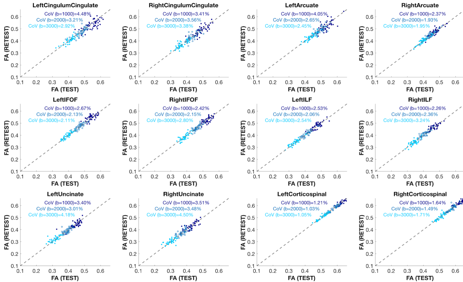
Figure S2. Mean tract FA HCP TEST-RETEST scatterplots. CoV calculated with the within-subject SD method ( Jones and Payne 1997 ; Synek 2008 )
