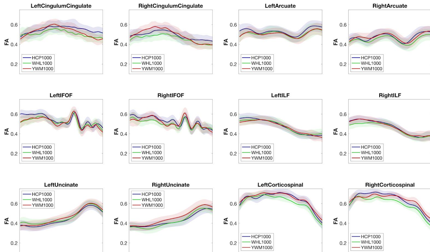
Figure S1b. Average FA profiles, b=1000 experiments, for six homologous white matter tracts.
