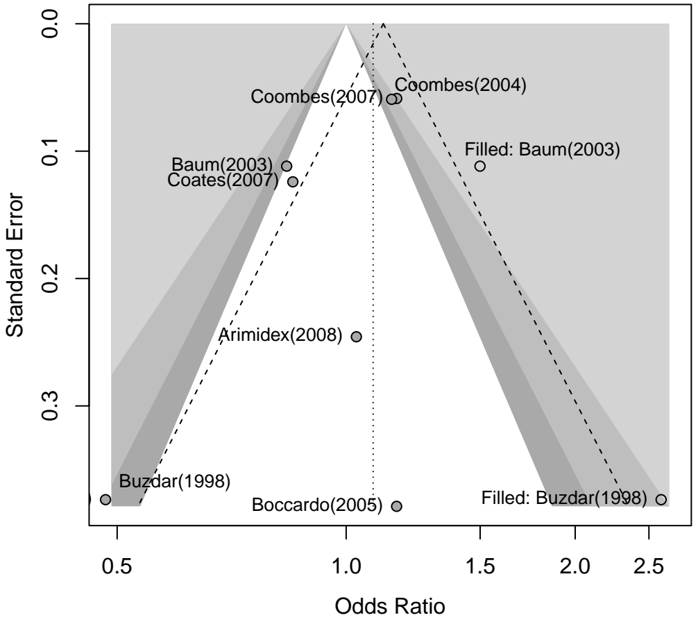
Figure S4. The contour-enhanced funnel plot for standard error by OR of CVEs.
