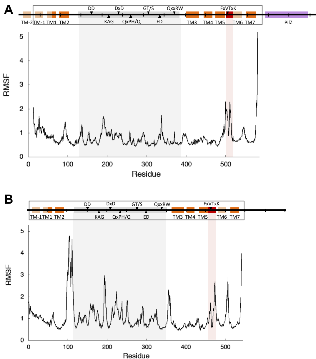
S7 Fig. Plot of RMSF from MD simulations. RMSF calculated over the last 50 ns of each simulation is plotted for (A) RsBcsA and (B) AtumCrdS. Simulations were unrestrained during production phase (having had restraints placed on them during the optimisation phase). Secondary structure schematic from Fig. 1A and B is displayed above each plot for reference with TM channel helices coloured dark orange, other TM helices light orange, the gating loop in red and the cytosolic domain in grey (referenced in Supplementary discussion).
