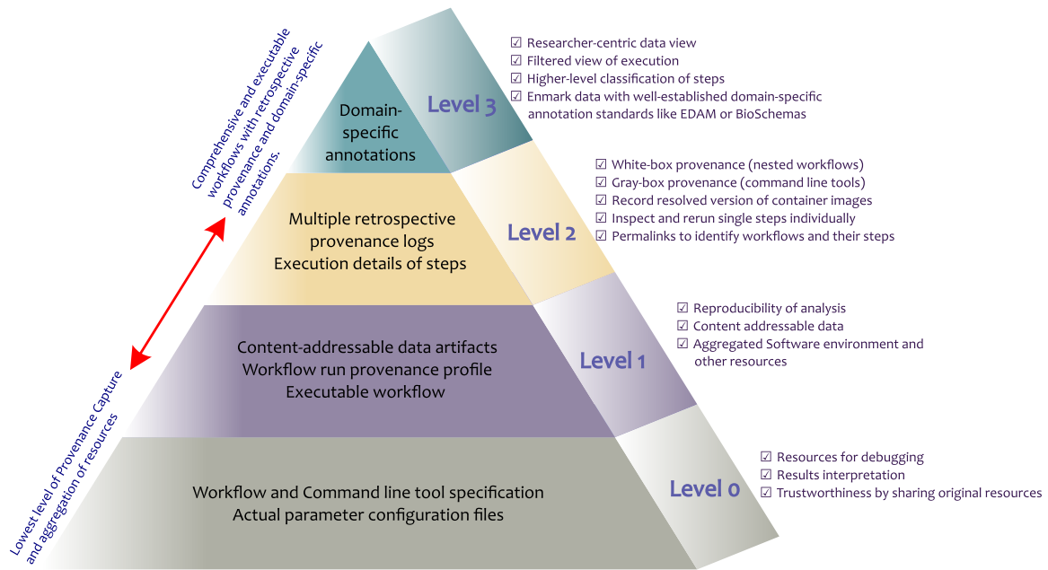
Figure 1. Levels of Provenance and resource sharing and their applications
