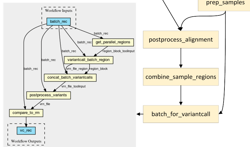
Figure 8. Visual representation of the bcbio somatic variant calling workflow (Adapted from [135]) and the subworkflow images are generated by CWL viewer.
