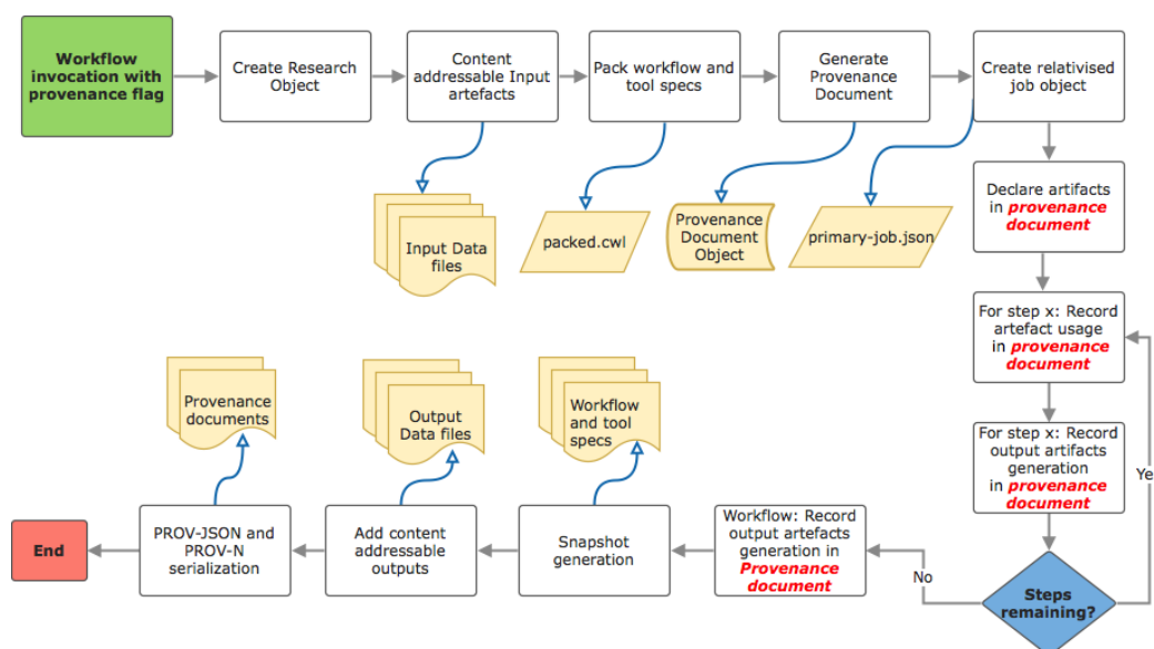
Figure 5. High level process flow representation of retrospective provenance capture
