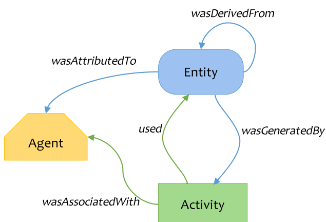
Figure 3. Core concepts of the PROV Data Model. Adapted from W3C PROV Model Primer [86].
