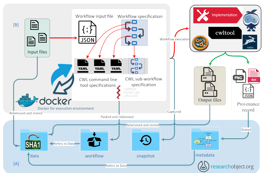
Figure 4. Schematic representation of the aggregation and links between the components of a given workflow enactment. Layers of execution are separated for clarity. The workflow specification and command line tool specifications are described using CWL. Each individual command line tool specification can optionally interact with Docker to satisfy software dependencies. [A] The RO layer shows the structure of the RO including its content and interactions with different components in the RO and [B] the CWL layer.
