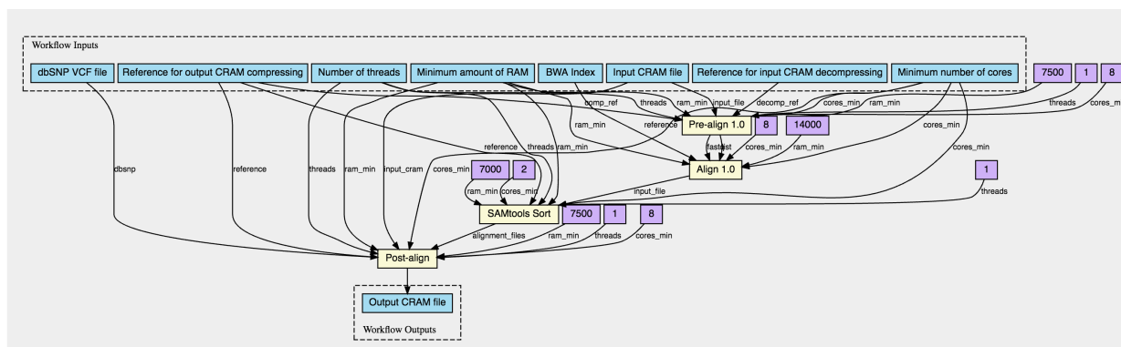
Figure 7. Alignment workflow representation generated by CWL viewer.
