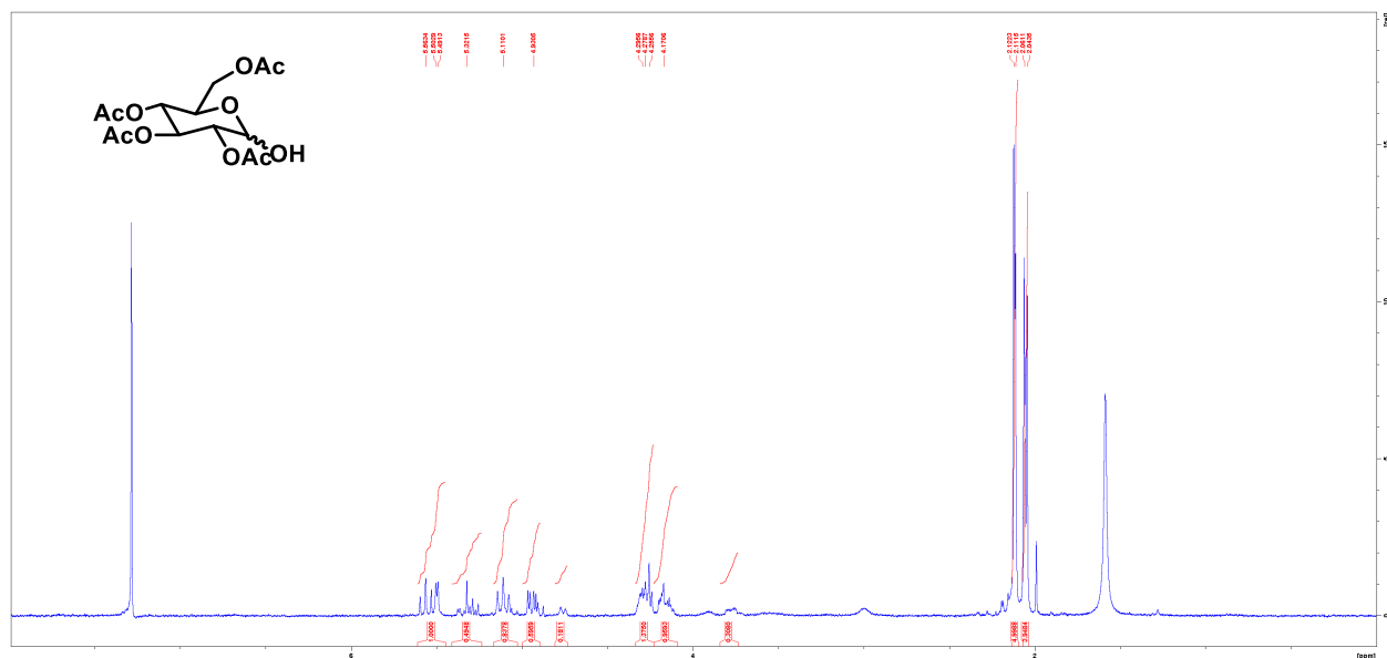
Figure S2. ^1\text{H} NMR (300 MHz, \text{CDCl}_3 ) of anomeric OH-deprotected peracetylated glycans S.2.
