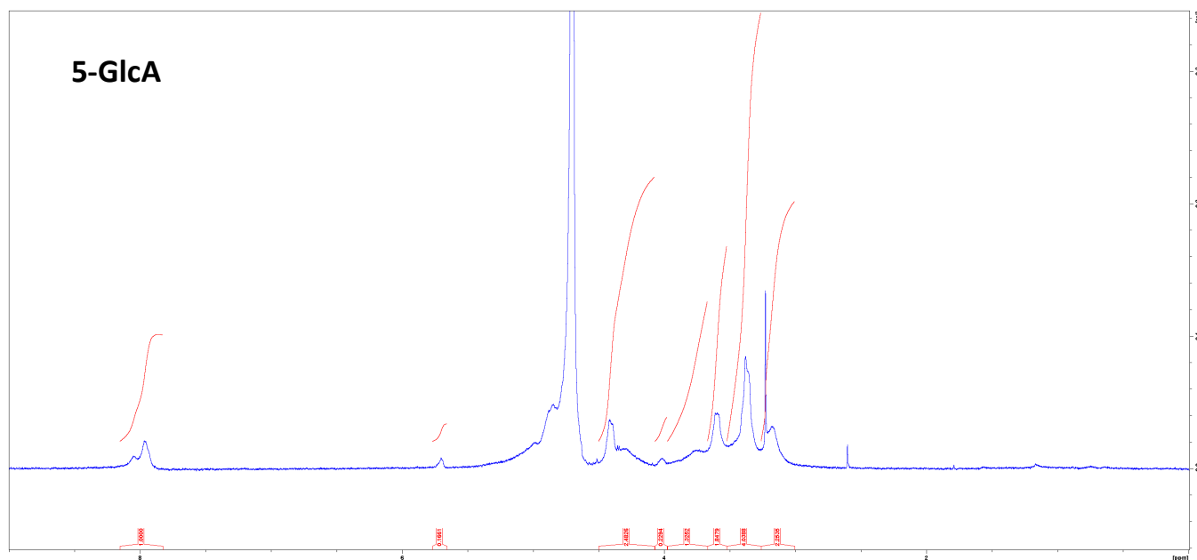
Figure S12. ^1\text{H} NMR (300 MHz, \text{D}_2\text{O} ) of glucuronic acid glycopolymer 5-GlcA .
