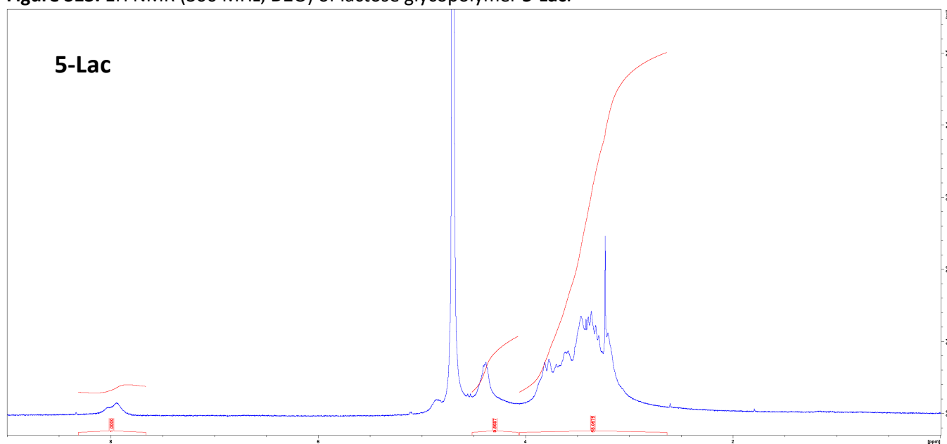
Figure S13. ^1\text{H} NMR (300 MHz, \text{D}_2\text{O} ) of lactose glycopolymer 5-Lac .
