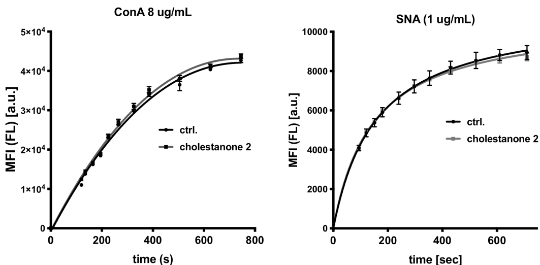
Figure S25. Binding of ConA and SNA to RBCs with pre-treatment with alkynyl cholestanone 2 (associated with Figure 4).
