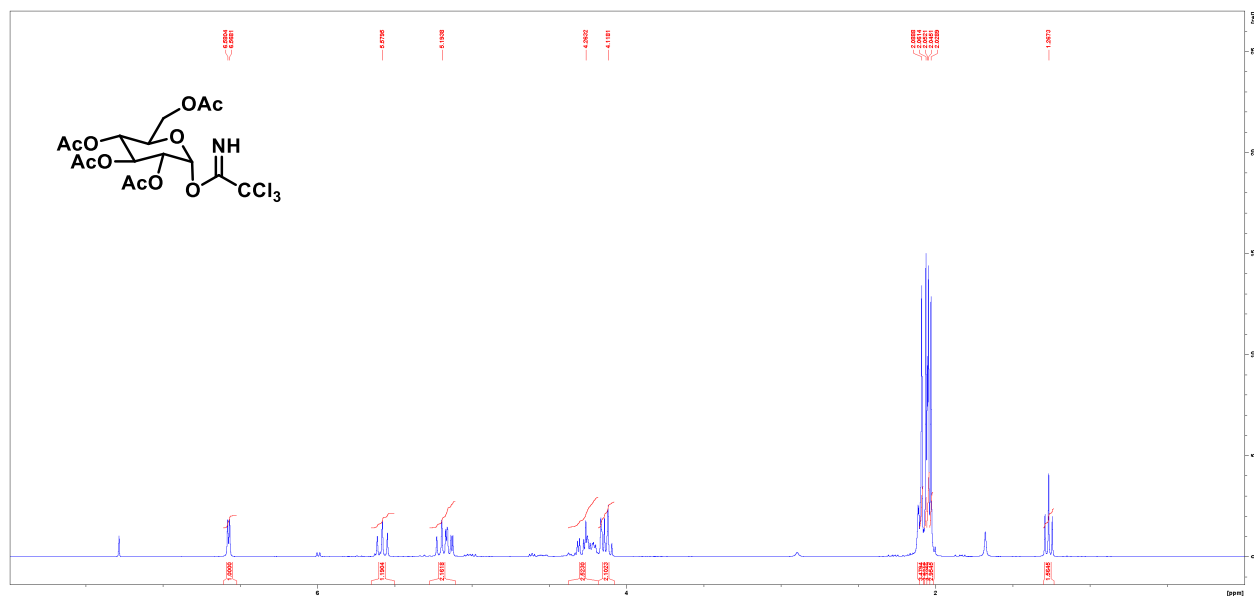
Figure S3. ^1\text{H} NMR (300 MHz, \text{CDCl}_3 ) of anomeric TCA glycosides S.3 .
