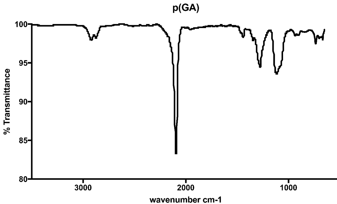
Figure S16. IR spectrum of pGA polymer 4.
