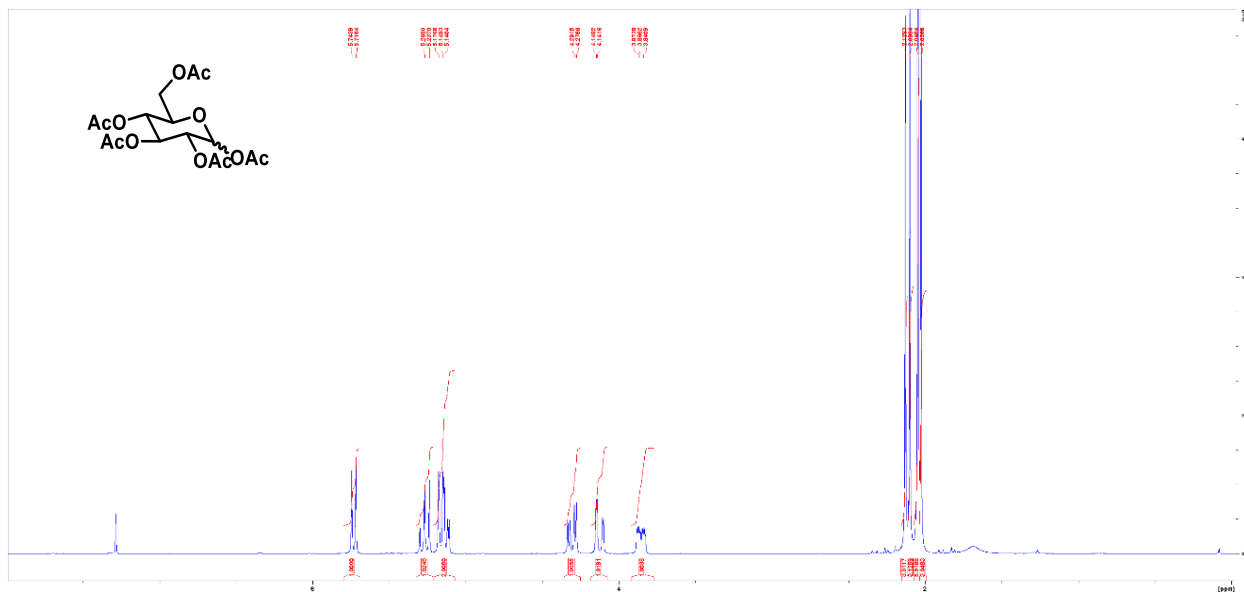
Figure S1. ^1\text{H} NMR (300 MHz, \text{CDCl}_3 ) of peracetylated glycans S.1.
