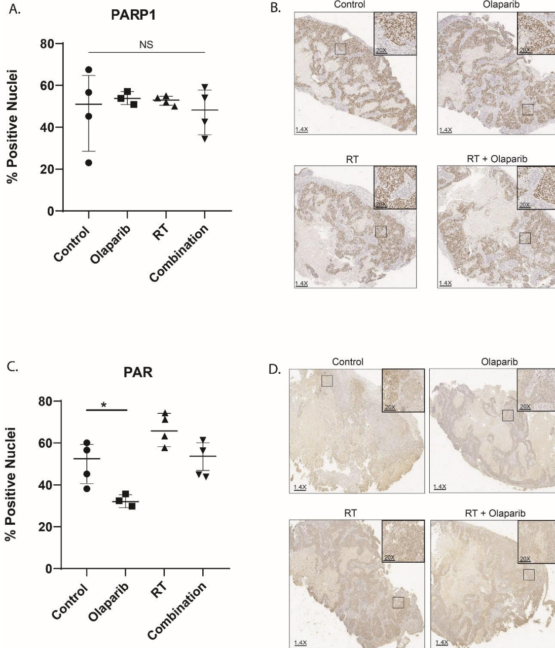
Supplemental Figure 4: Total PARP1 levels do not change with treatment but PAR levels are decreased by PARPi. Total levels of PARP1 were assessed in tumors from mice treated with olaparib. Olaparib treatment did not affect PARP1 protein expression by IHC in olaparib-alone, RT alone, or combination treated animals (A). Representative images of PARP1 staining are shown for all treatment conditions (B). PAR levels were, however, significantly decreased in the animals treated with olaparib alone (C). Representative images of PAR staining are shown for all treatment conditions (D). (NS: not significant, * p < 0.05 )
