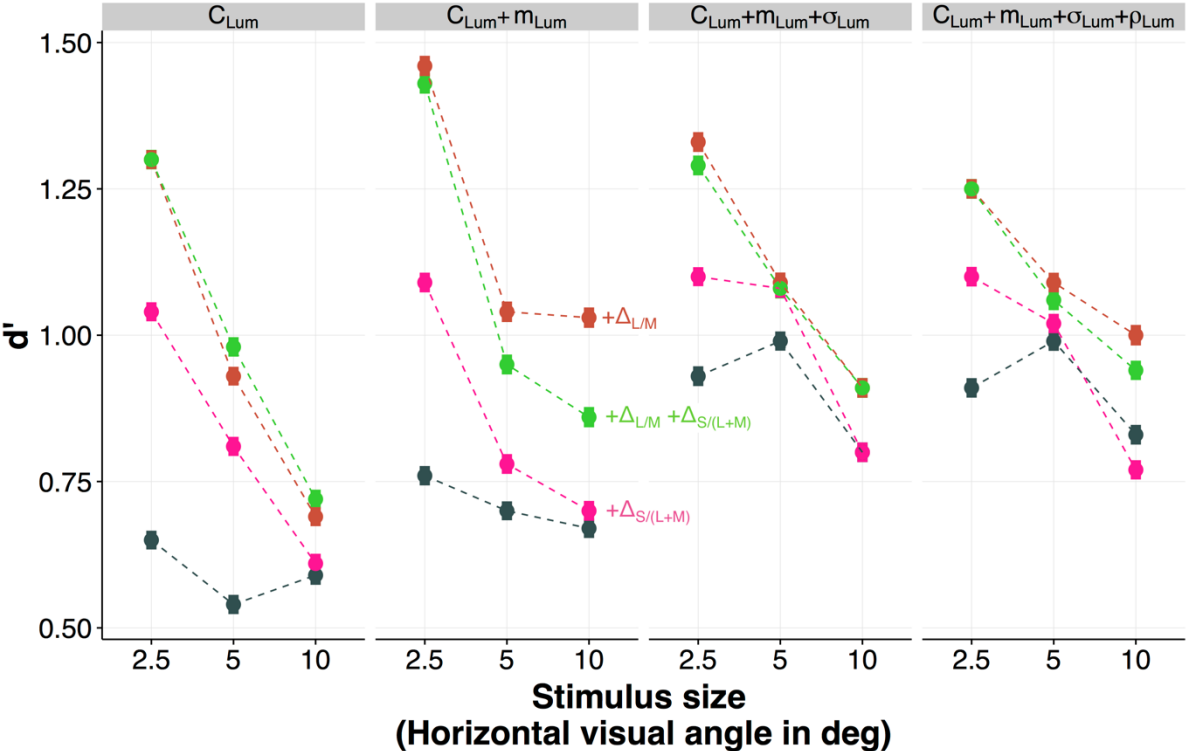
Figure S3 –Summary of classifiers performance expressed in terms of d' values. Intervals correspond to lower and upper 95 th percentile confidence interval based on parametric bootstrap simulations (n=1000).
