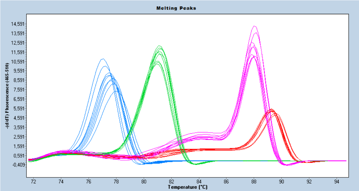
Figure S1: Melting curves for HPRT (blue), Id1 (red), Id2 (green), Id3 (pink) for unstimulated C2C12 cells and cells stimulated with BMP2 (1nM) with and without arginine.
