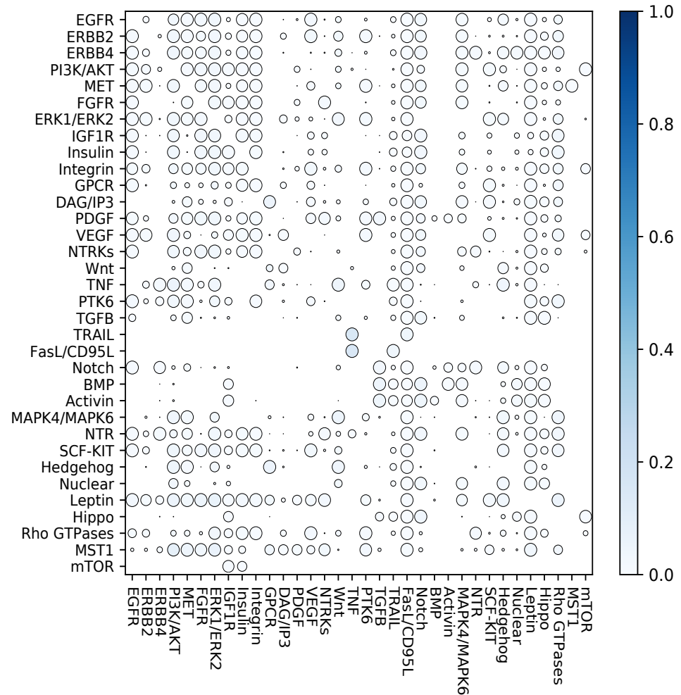
Influence Score s_{50}
