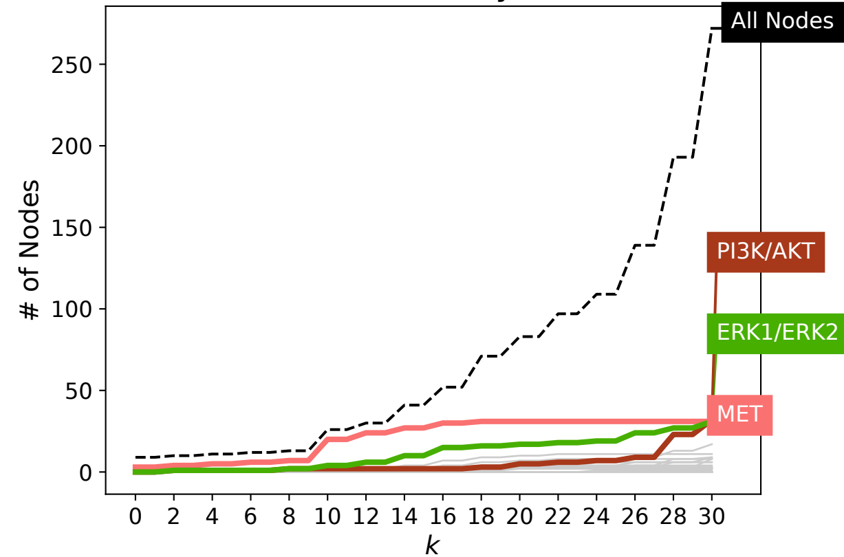
Source Pathway MST1
