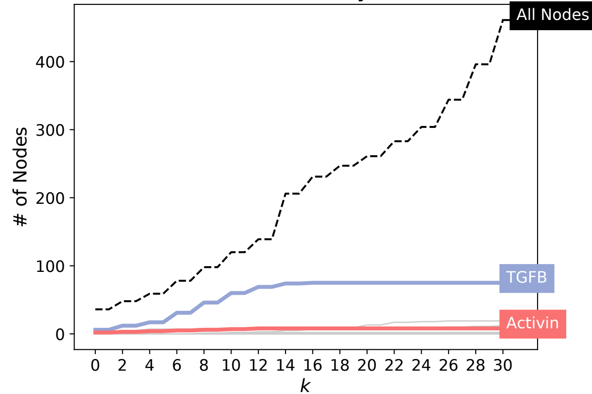
Source Pathway BMP
