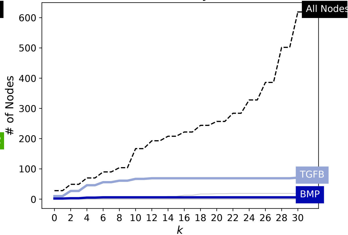
Source Pathway Activin
