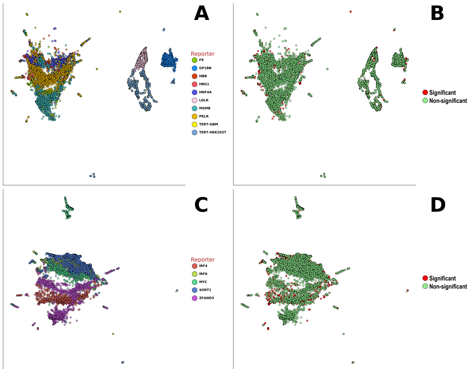
Supplementary Figure 1. SNVs in promoters (A, B) and in enhancers (C, D) in the two-dimensional UMAP space. The plots illustrate clear separation of reporters, while significant regulatory SNVs are non-trivially mixed with the non-significant SNVs. The SNVs of the MYC reporter are arranged in two distant clusters, which is probably linked to its unusual behavior in holdout tests.
