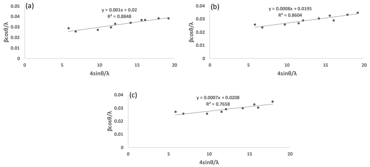
Figure 1: Williamson-Hall plots of PbS at (a) 250, 300, 400 °C
