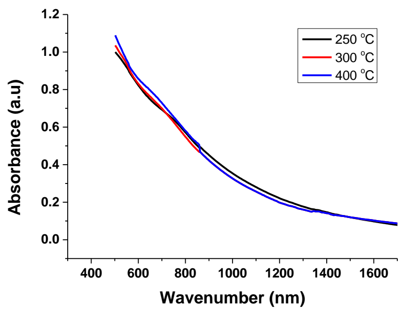
Figure 2: Uv-vis-nir of PbS at 250, 300, 400 °C
