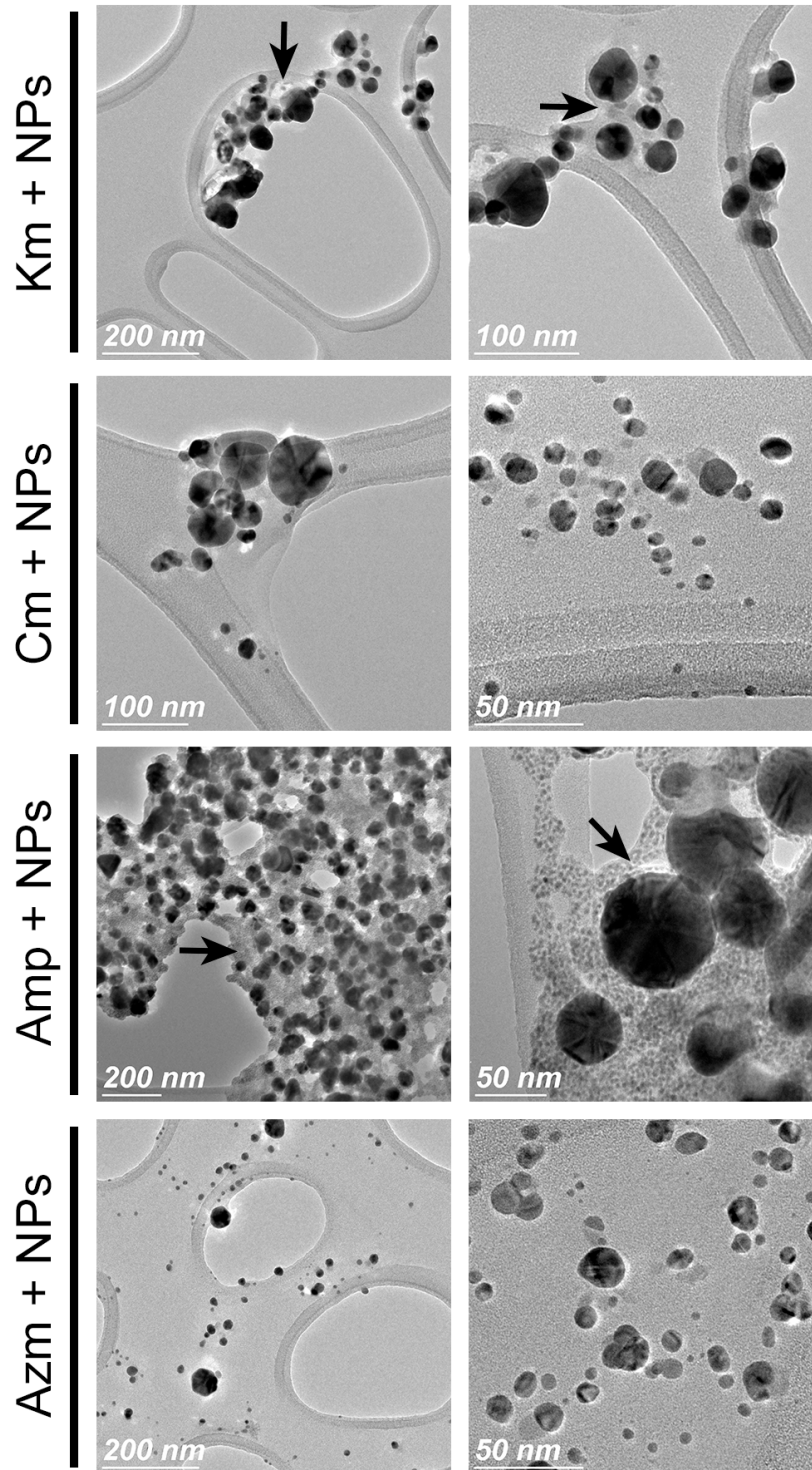
S4 Figure. TEM images of the combined AgNPs and antibiotic treatments. An aggregative effect was observed for Km + AgNPs and Amp + AgNPs combinations (marked with arrows). Images were taken after 24 hours of incubation.
