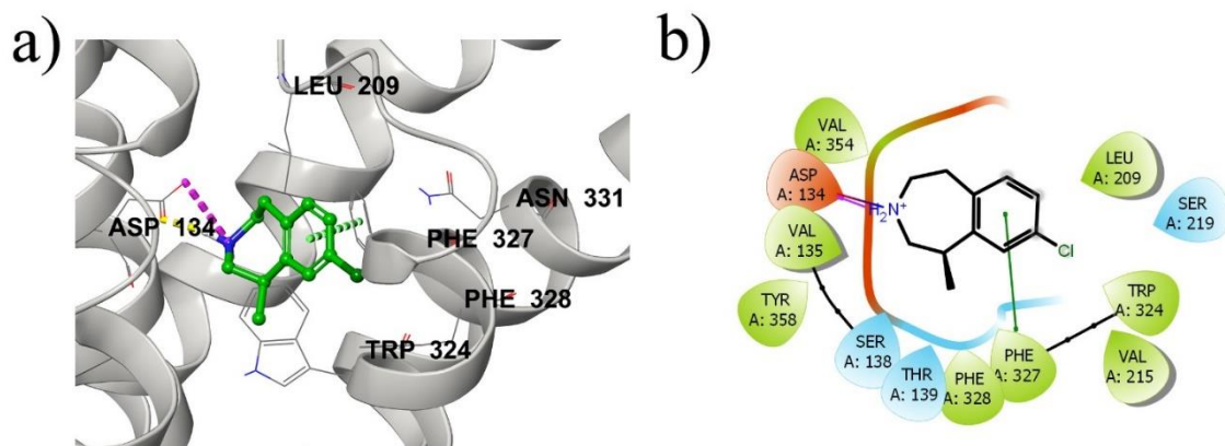
Figure S1: Interaction profile of known drug lorcaserin with 5HT 2C receptor after docking studies depicted in both 3D (left side; Hydrogen bonds (yellow), salt bridge (magenta) and \pi - \pi (green) interactions as shown in dotted lines) and 2D (right side) forms
