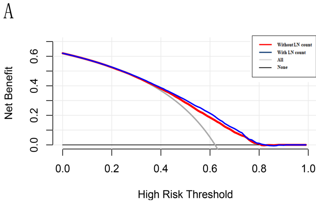
Fig S1. Decision curve analyses of the 5-year CSS (A) and OS (B) predictions. The dashed lines indicate the net benefit of using the nomograms based on with lymph node count (solid full line) and without lymph node count (solid full line). The assumption that all of the patients will die is shown with a grey line, and the assumption that all of the patients will survive is indicated with a black line. Threshold probability = 1 - predicted 5-year CSS and OS.
