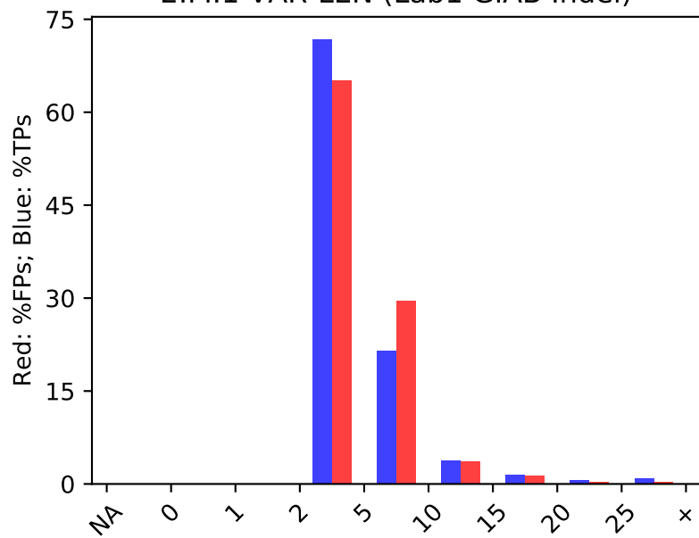
2.M.1 VAR-LEN (Lab1 GIAB Indel)
