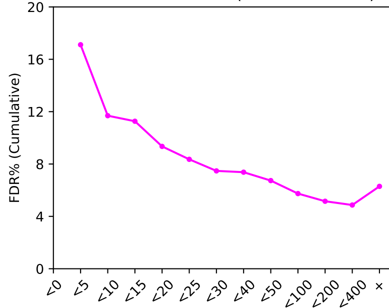
2.L.4 NEARBY-VARS (Lab1 GIAB Indel)
