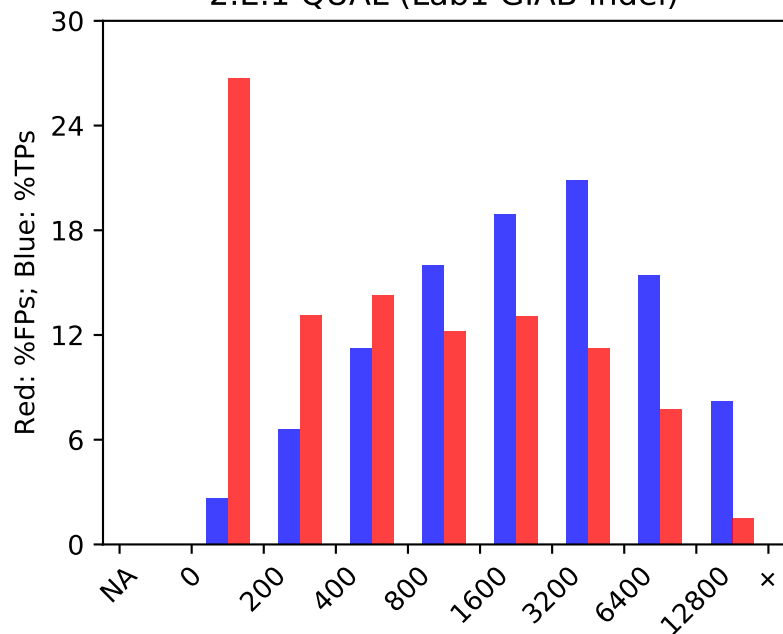
2.E.1 QUAL (Lab1 GIAB Indel)
