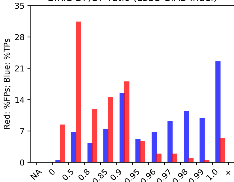
2.K.1 DP/DP ratio (Lab1 GIAB Indel)
