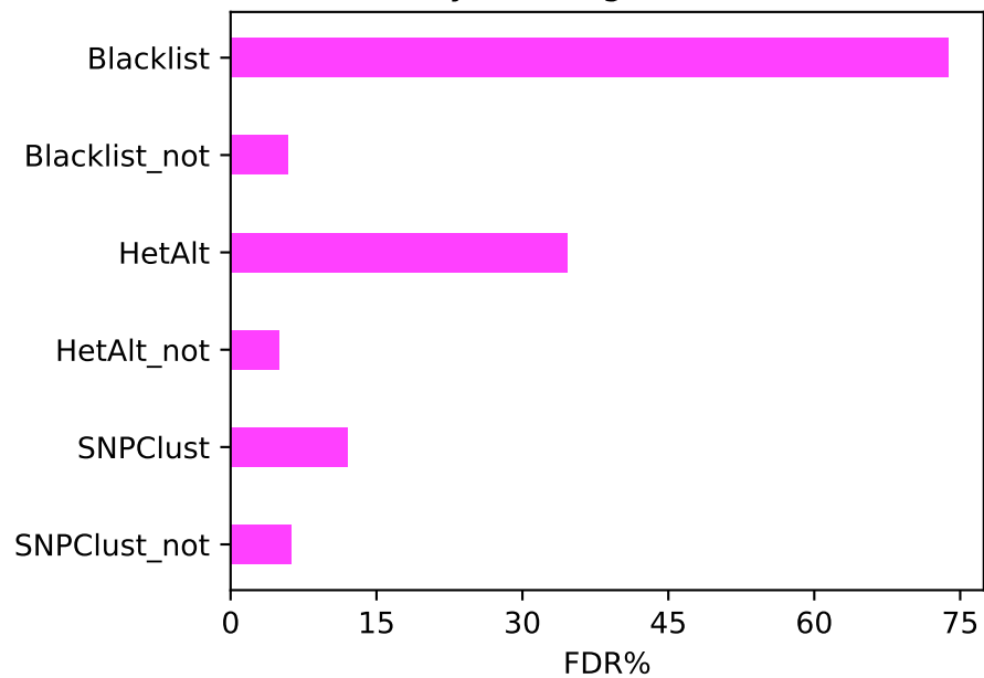
2.N.2 Binary warnings (Lab1 GIAB Indel)
