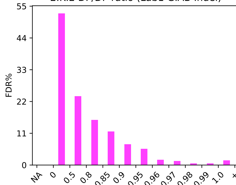
2.K.2 DP/DP ratio (Lab1 GIAB Indel)
