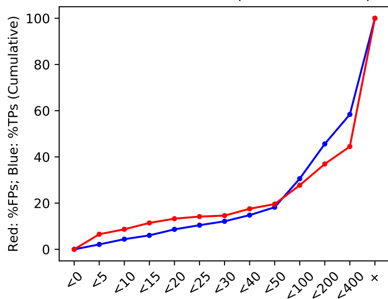
2.L.3 NEARBY-VARS (Lab1 GIAB Indel)
