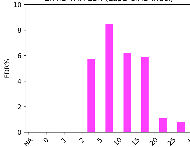
2.M.2 VAR-LEN (Lab1 GIAB Indel)
