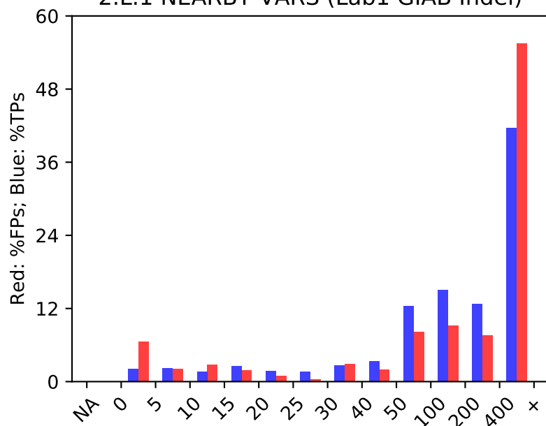
2.L.1 NEARBY-VARS (Lab1 GIAB Indel)
