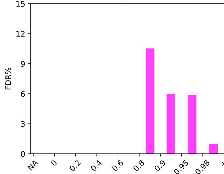
2.D.2 ABhom (Lab1 GIAB Indel)
