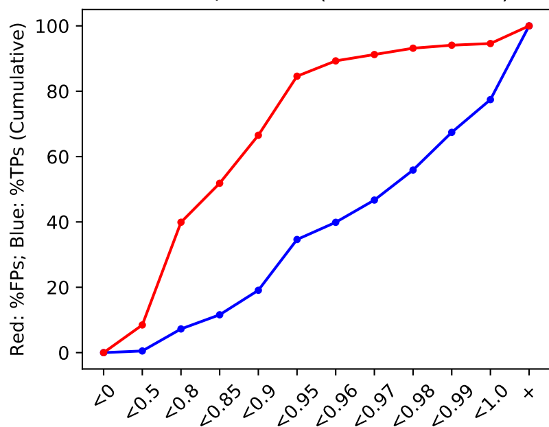
2.K.3 DP/DP ratio (Lab1 GIAB Indel)
