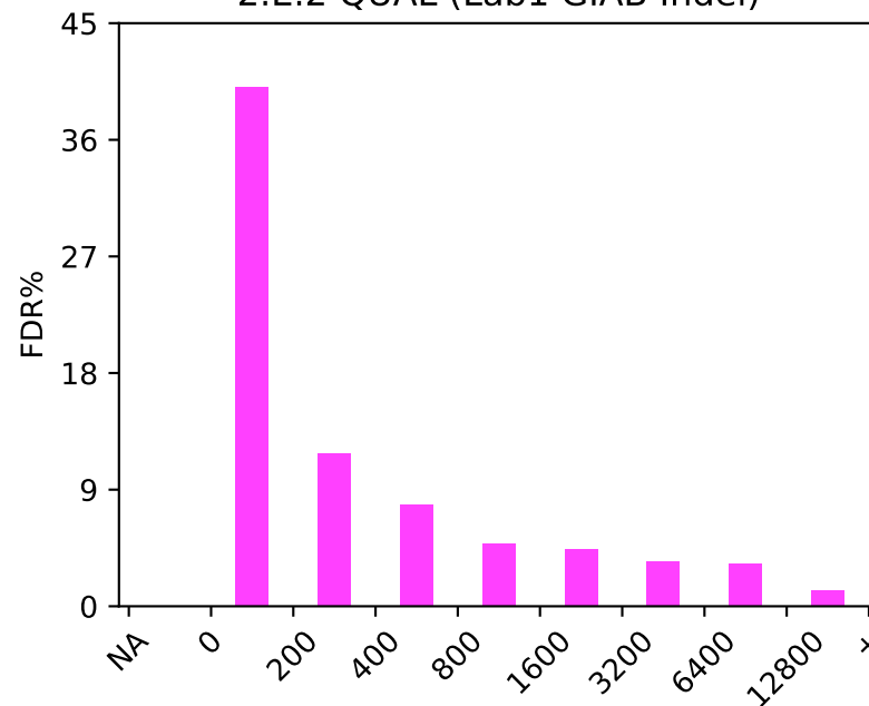
2.E.2 QUAL (Lab1 GIAB Indel)
