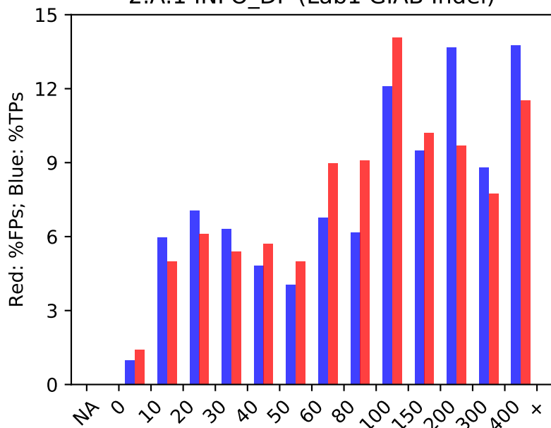
2.A.1 INFO_DP (Lab1 GIAB Indel)
