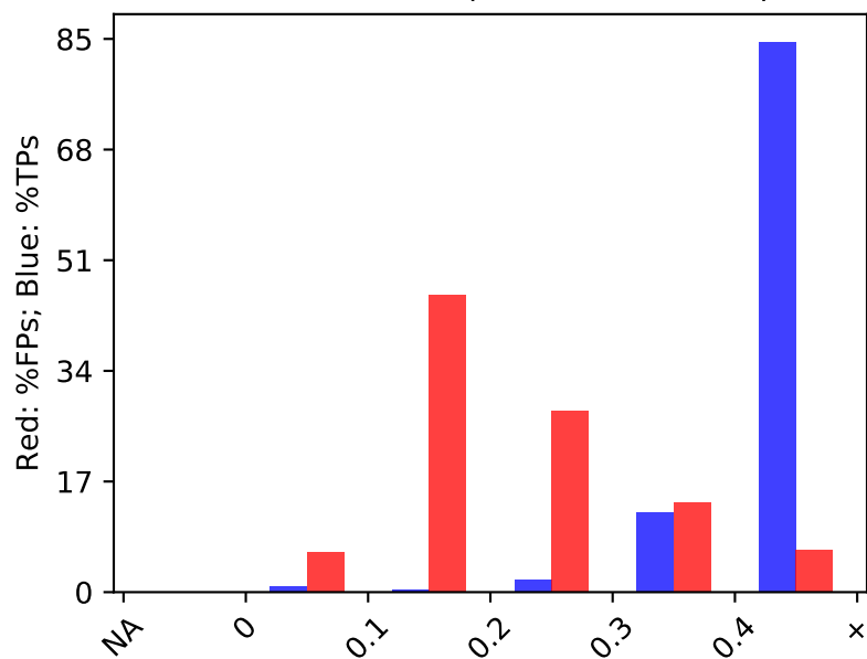
2.C.1 ABnorm (Lab1 GIAB Indel)
