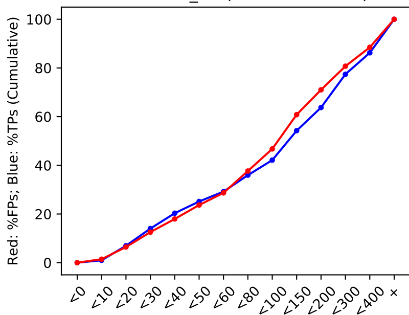
2.A.3 INFO_DP (Lab1 GIAB Indel)
