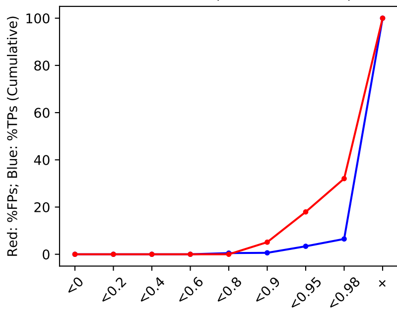
2.D.3 ABhom (Lab1 GIAB Indel)
