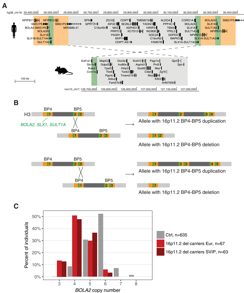
Figure 1. The 16p11.2 and BOLA2 Locus Architecture
