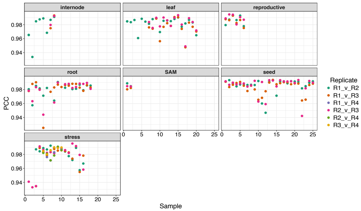
Figure S1: Biological Replicate Pearson's Correlation Coefficients
