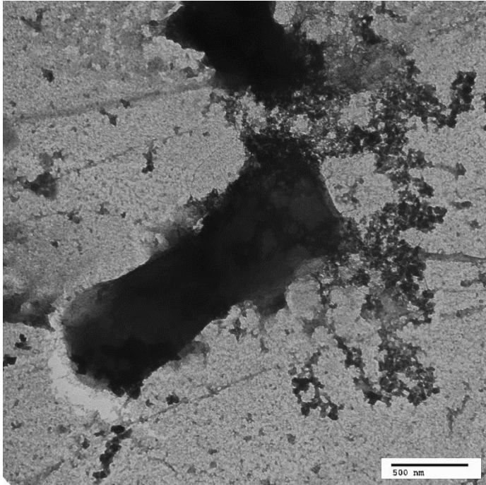
AF11: Shigella flexneri serotype 3a
