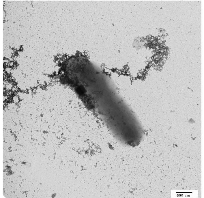
AF16: Shigella flexneri serotype 2a
