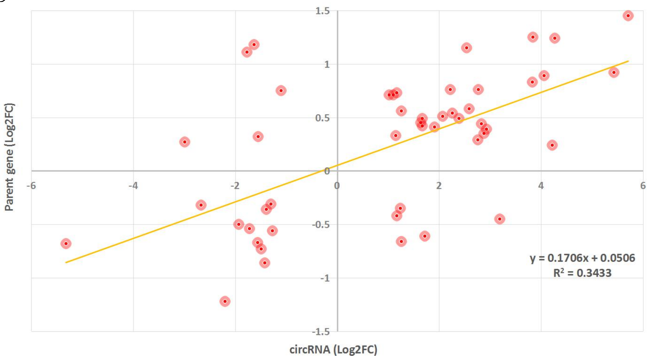
Fig. S4. Co-expression patterns of coding RNAs and three type of non-coding RNAs. (A) Equation of linear regression of fold-changes on log 2 -scale of the miRNAs ( |\log_2FC| \geq 1 ) and their target genes. (B) Equation of linear regression of fold-changes on log 2 -scale of the miRNAs ( |\log_2FC| \geq 1 ) and their target exonic-circRNAs ( |\log_2FC| \geq 1 ). (C) Equation of linear regression of fold-changes on log 2 -scale of the circRNAs ( |\log_2FC| \geq 1 ) and their host genes (FDR < 0.05).
