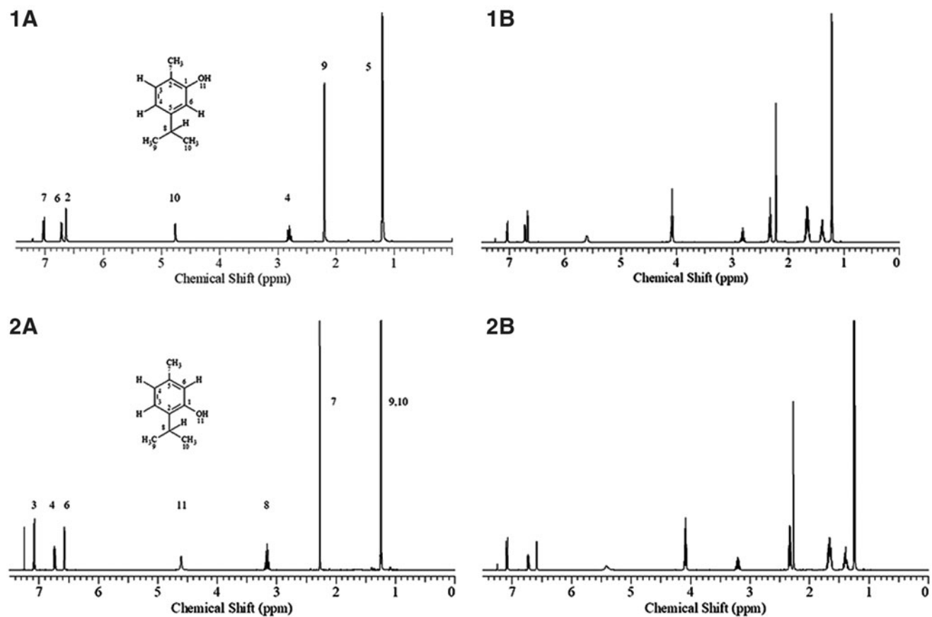
Supplementary Figure S1. (1-A) CAR structure and ^1\text{H} NMR spectrum of CAR. (1-B) ^1\text{H} NMR spectrum of CAR/PCL fibers. (2-A) THY structure and ^1\text{H} NMR spectrum of THY. (2-B) ^1\text{H} NMR spectrum of THY/PCL fibers. CAR, carvacrol; NMR, nuclear magnetic resonance; PCL, polycaprolactone; THY, thymol.
