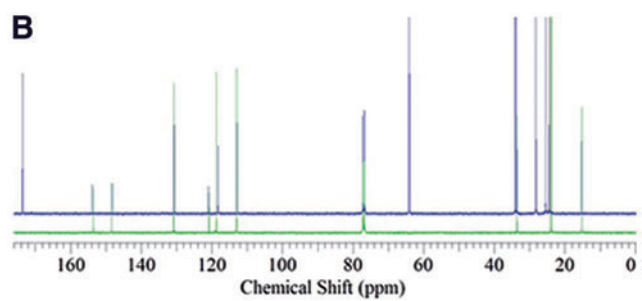
Supplementary Figure S2. (A) Full 13 C NMR spectrum of THY ( green line ) and THY/PCL mixture ( blue line ). (B) Full 13 C NMR spectrum of CAR ( green line ) and CAR/PCL mixture ( blue line ).
