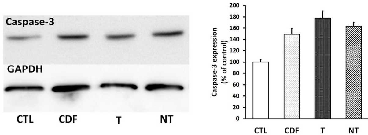
Figure S1. Western blot analysis and quantification of Caspase 3 with respect to GAPDH. The quantified data indicates the upregulation of Caspase-3 expression for targeted formulation SPIONs@FA-PAMAM-CDF (T) treatment than the control without treatment (CTL), cells treated with CDF, and non-targeted formulation SPIONs@PAMAM-CDF (NT) in HeLa cell line (GAPDH expression was used as the protein loading control).
