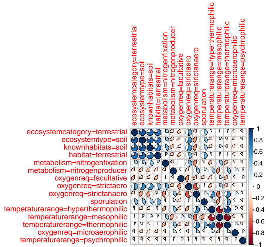
S1 Fig: The pairwise correlation between traits among species in the trait dataset. Note that some traits are highly correlated.
