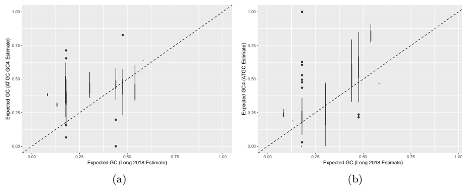
S12 Fig: We evaluate the use of polymorphisms as a proxy for mutation by comparing estimates for the few species present in both the polymorphism and mutation accumulation data. (a) Estimates based on all polymorphisms. (b) Estimates based on polymorphisms at fourfold degenerate sites. Here we see selection/BGC appears to bias the polymorphism estimates when mutation is extremely biased towards AT.
