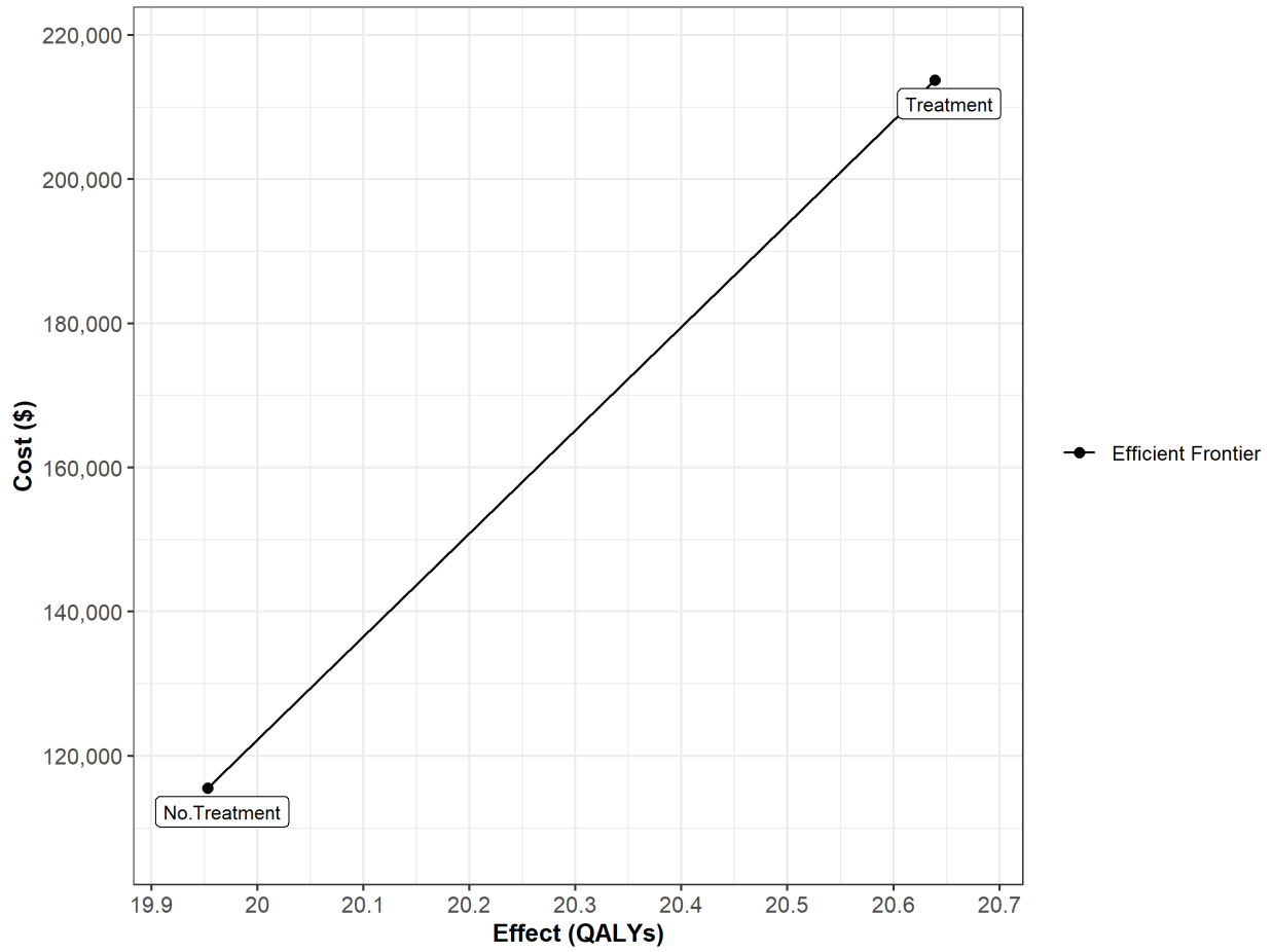
Figure 5.2: Cost-effectiveness frontier
