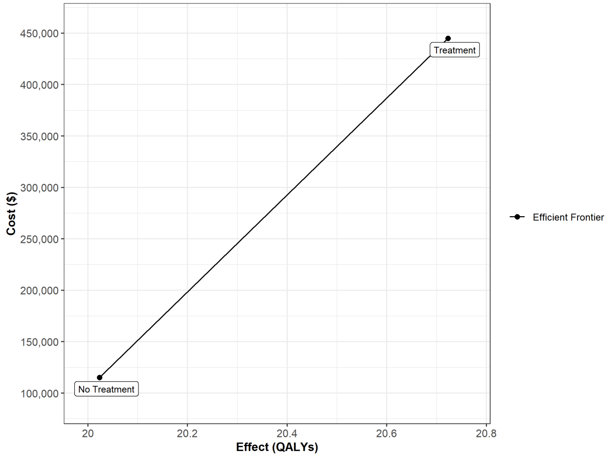
Figure 5.9: Cost-effectiveness frontier.
