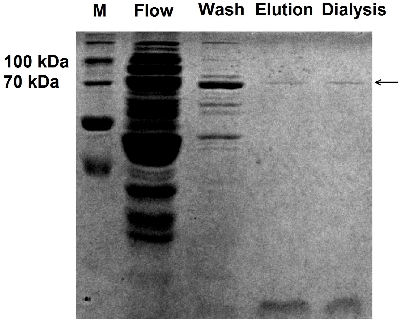
Supplemental Fig. S3. Expression and purification of the recombinant His-Blp1 2652-3362 C-terminal fragment. Fractions of flow-through, column washing, elution and dialysis in PBS buffer were fractionated in 12% SDS-PAGE. The position of His-Blp1 2652-3362 C-terminal fragment is indicated by the arrow. The positions of standard molecular mass markers (PageRuler™ Prestained Protein Ladder (Thermo Fisher Scientific)) are shown on the left.
