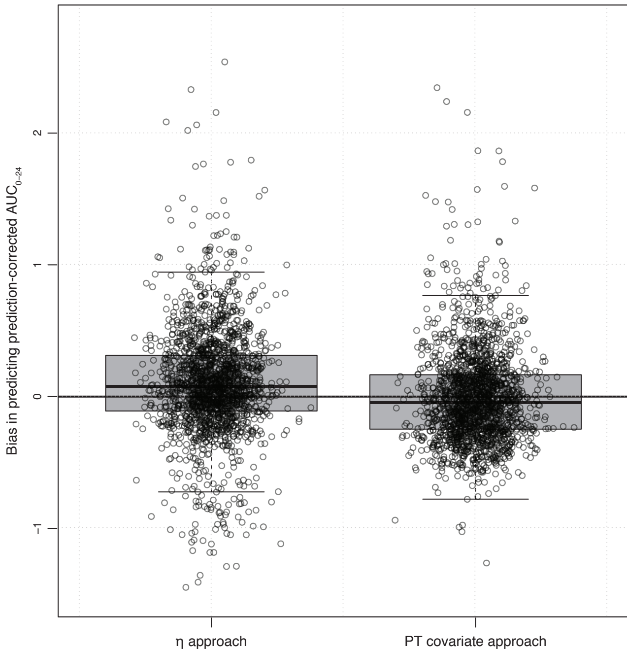
Figure S3 Absolute bias of the \eta and PT covariate approaches in predicting prediction-corrected AUC_{0-24} .
