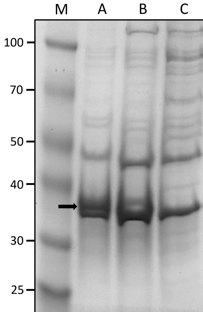
Supplementary Figure S1. SDS-PAGE analysis for OMP profiles of reference strain K. pneumoniae CIP53153 (lane A), K. pneumoniae 11978 (lane B) and K. pneumoniae MAS9 (lane C). Lane M, molecular size marker are indicated in kilodaltons (on the left). Black arrow indicates the position of OmpK36, that is missing in K. pneumoniae 11978 and K. pneumoniae MAS9.
